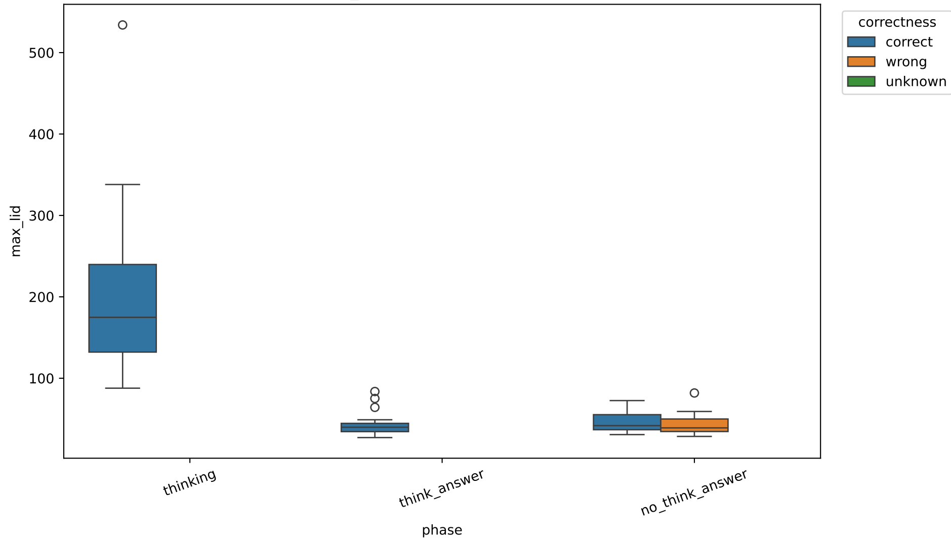
Exp C max_lid by correctness, 32B, layer 13
