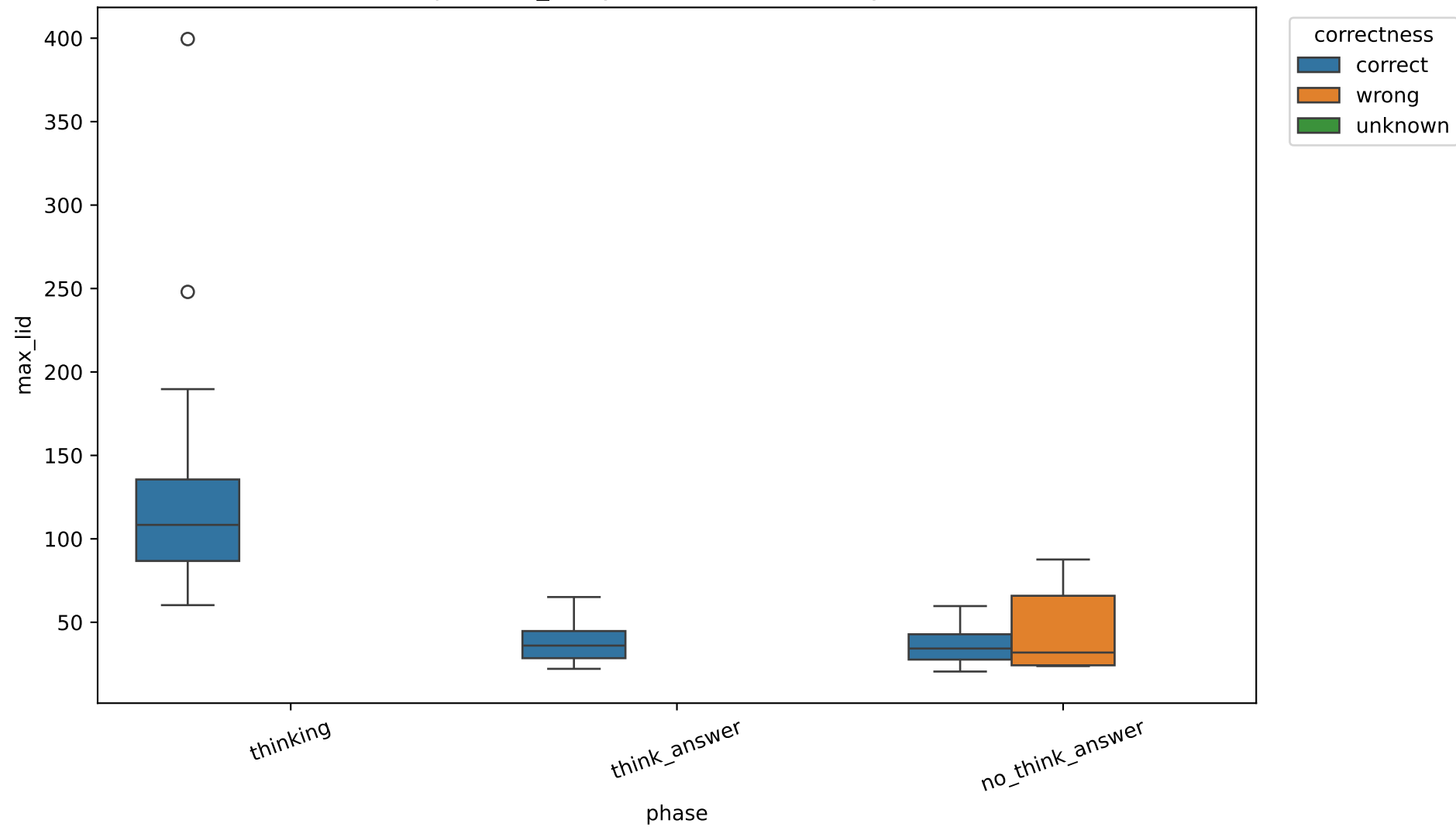
Exp C max_lid by correctness, 32B, layer 20
