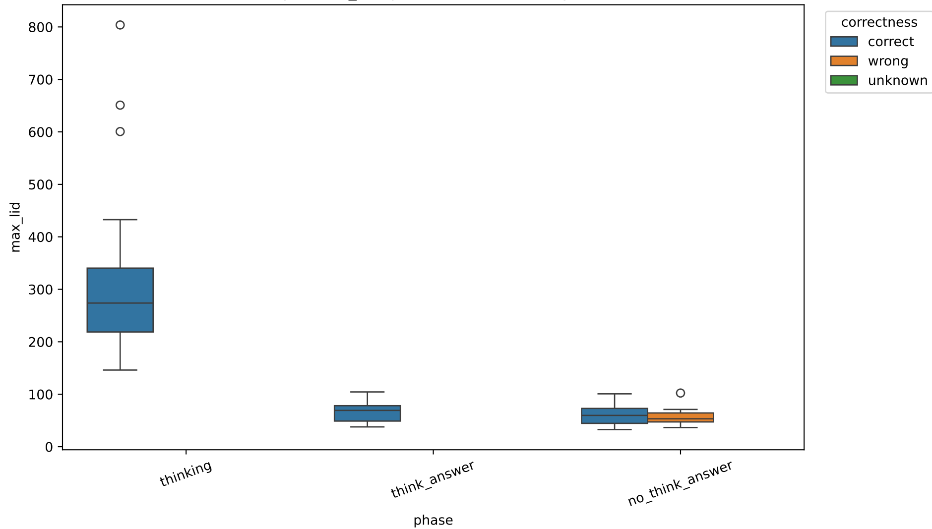
Exp C max_lid by correctness, 32B, layer 6
