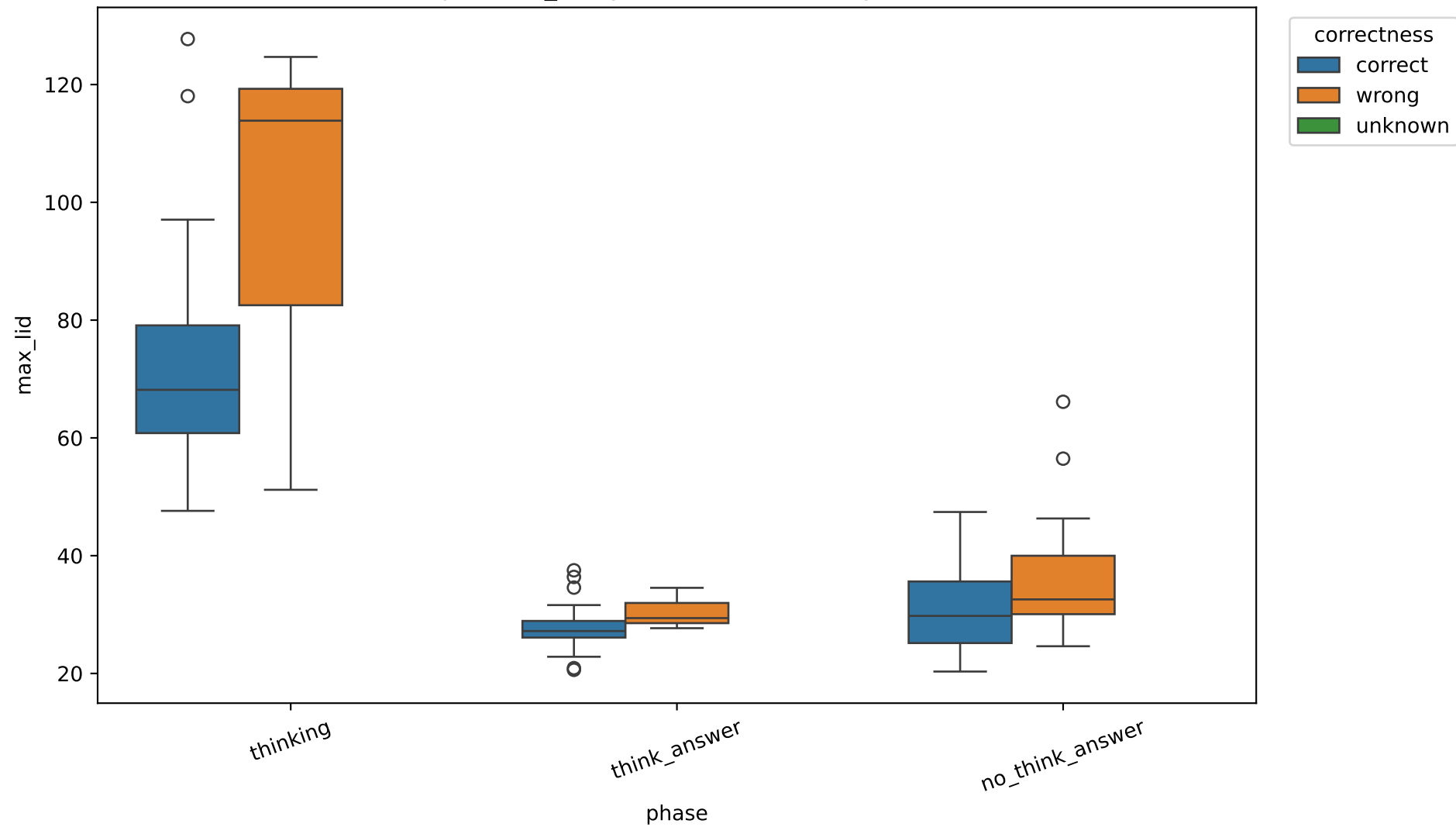
Exp C max_lid by correctness, 8B, layer 13
