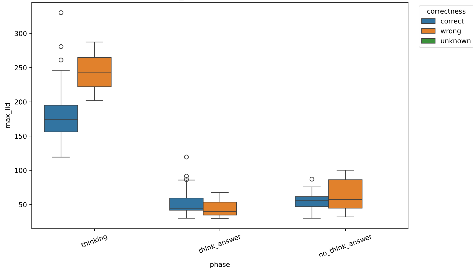
Exp C max_lid by correctness, 8B, layer 6
