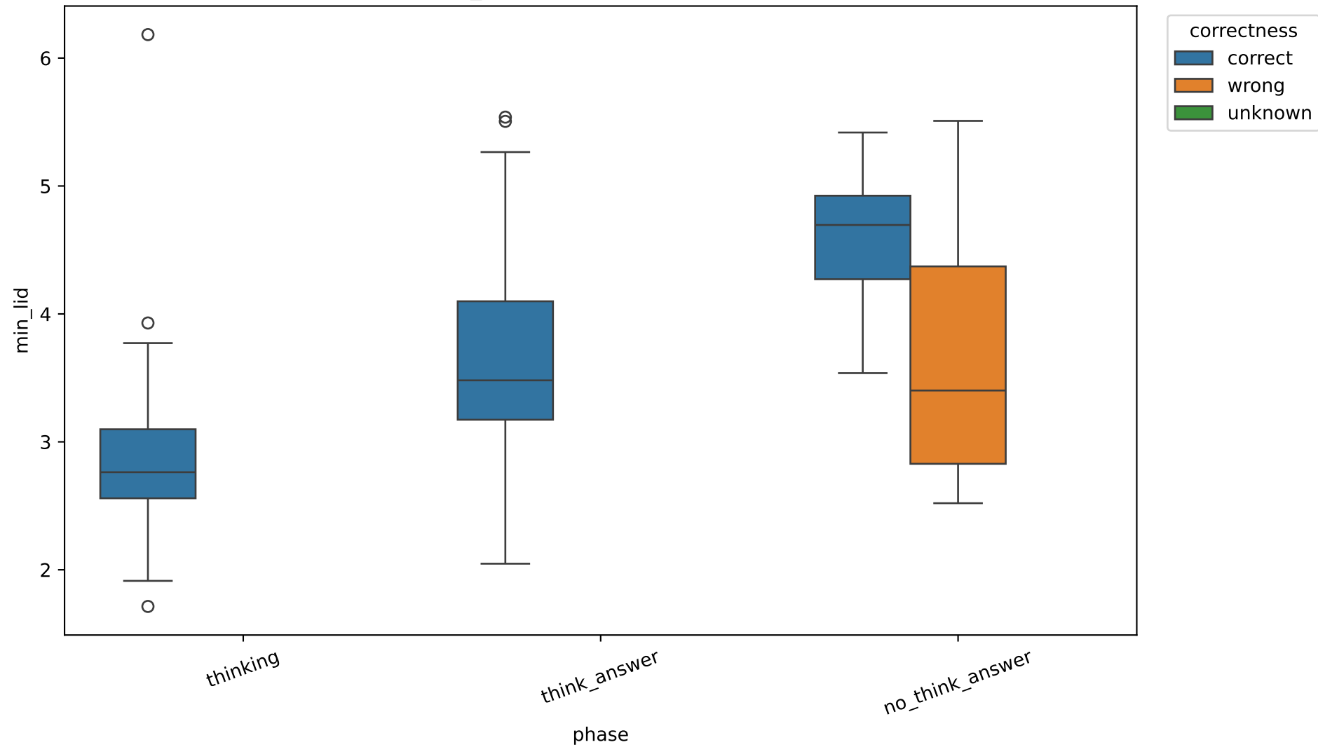
Exp C min_lid by correctness, 14B, layer 13
