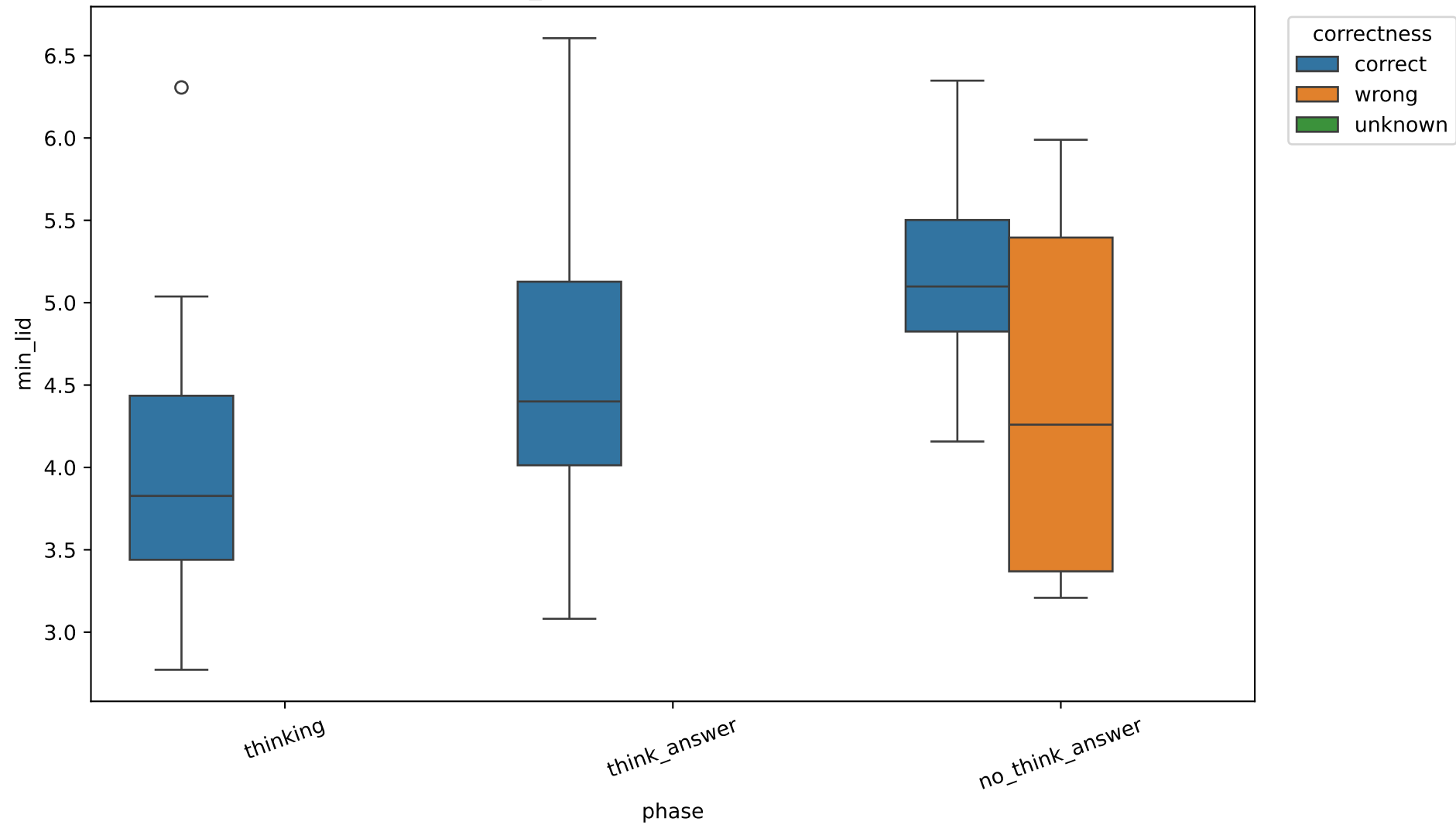
Exp C min_lid by correctness, 14B, layer 20
