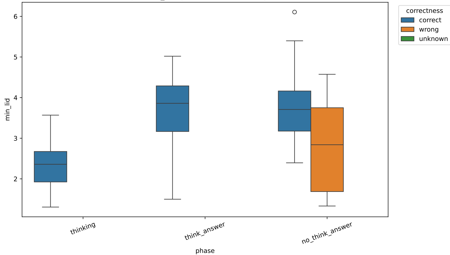
Exp C min_lid by correctness, 32B, layer 13
