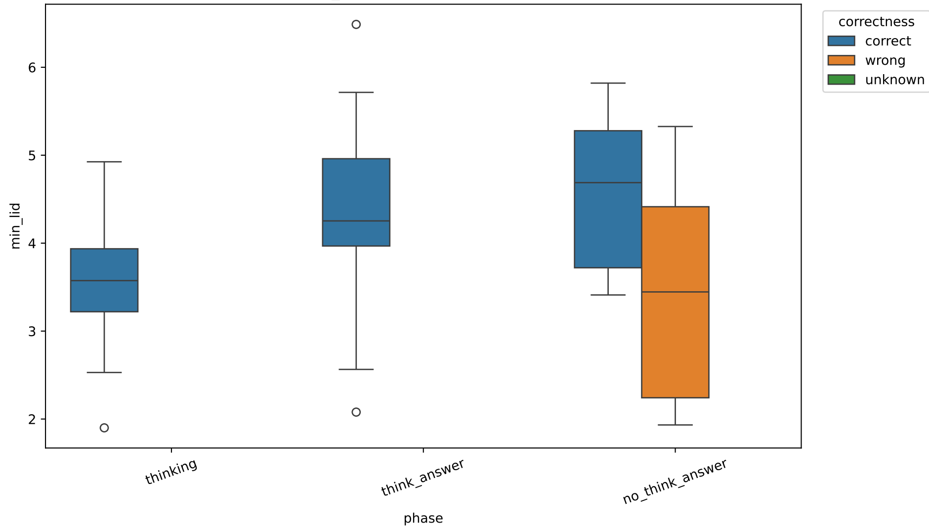
Exp C min_lid by correctness, 32B, layer 20
