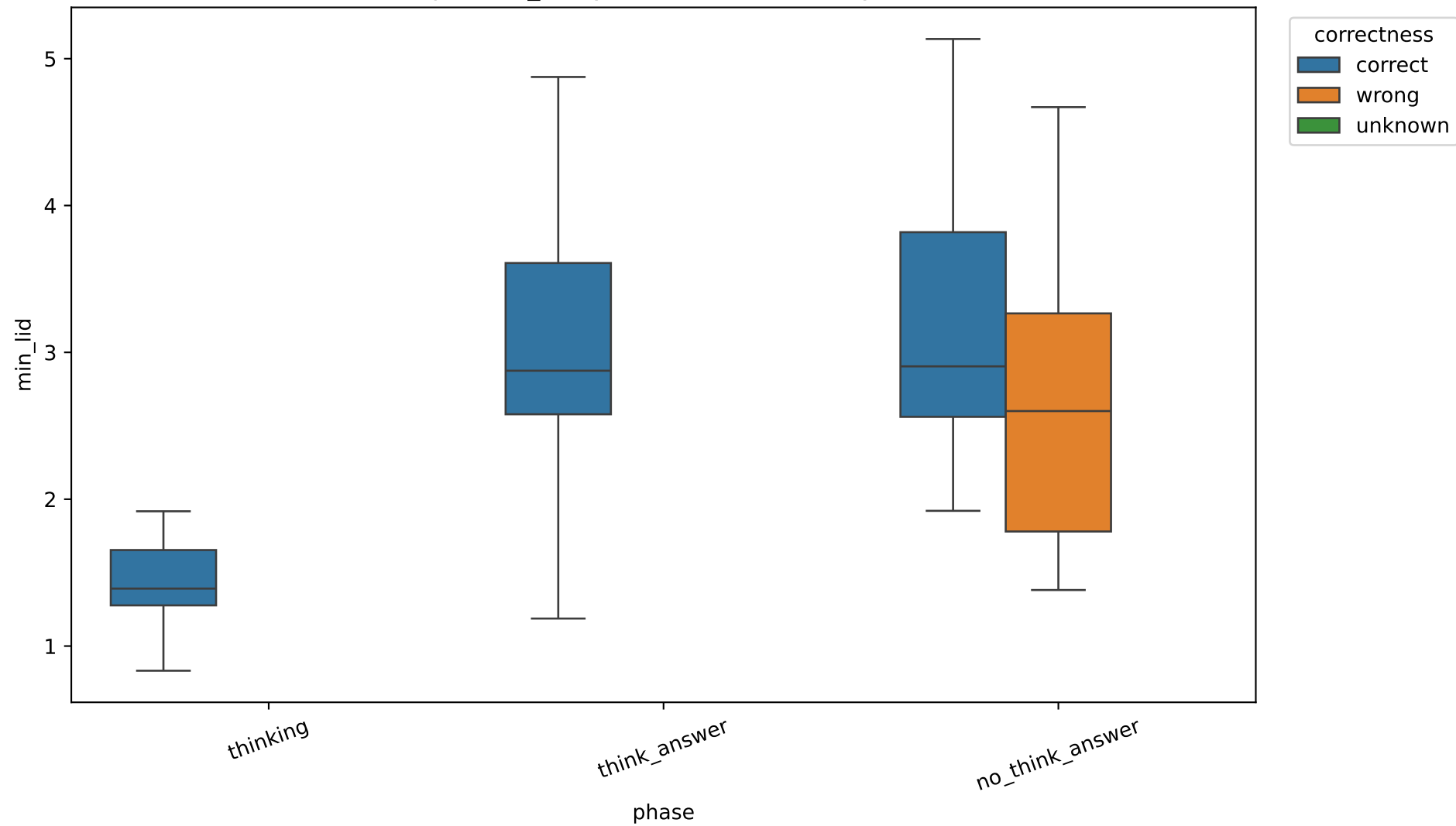
Exp C min_lid by correctness, 32B, layer 6
