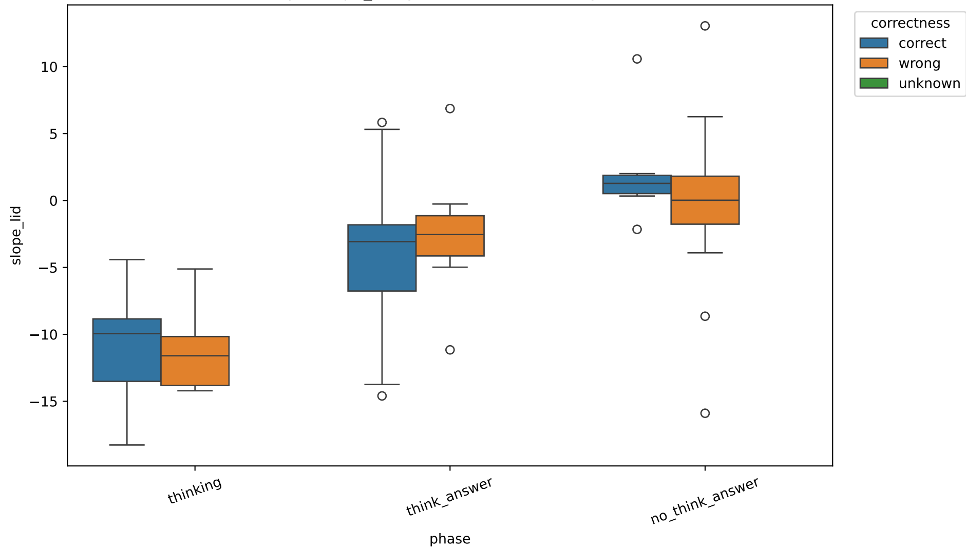
Exp C slope_lid by correctness, 1.7B, layer 6
