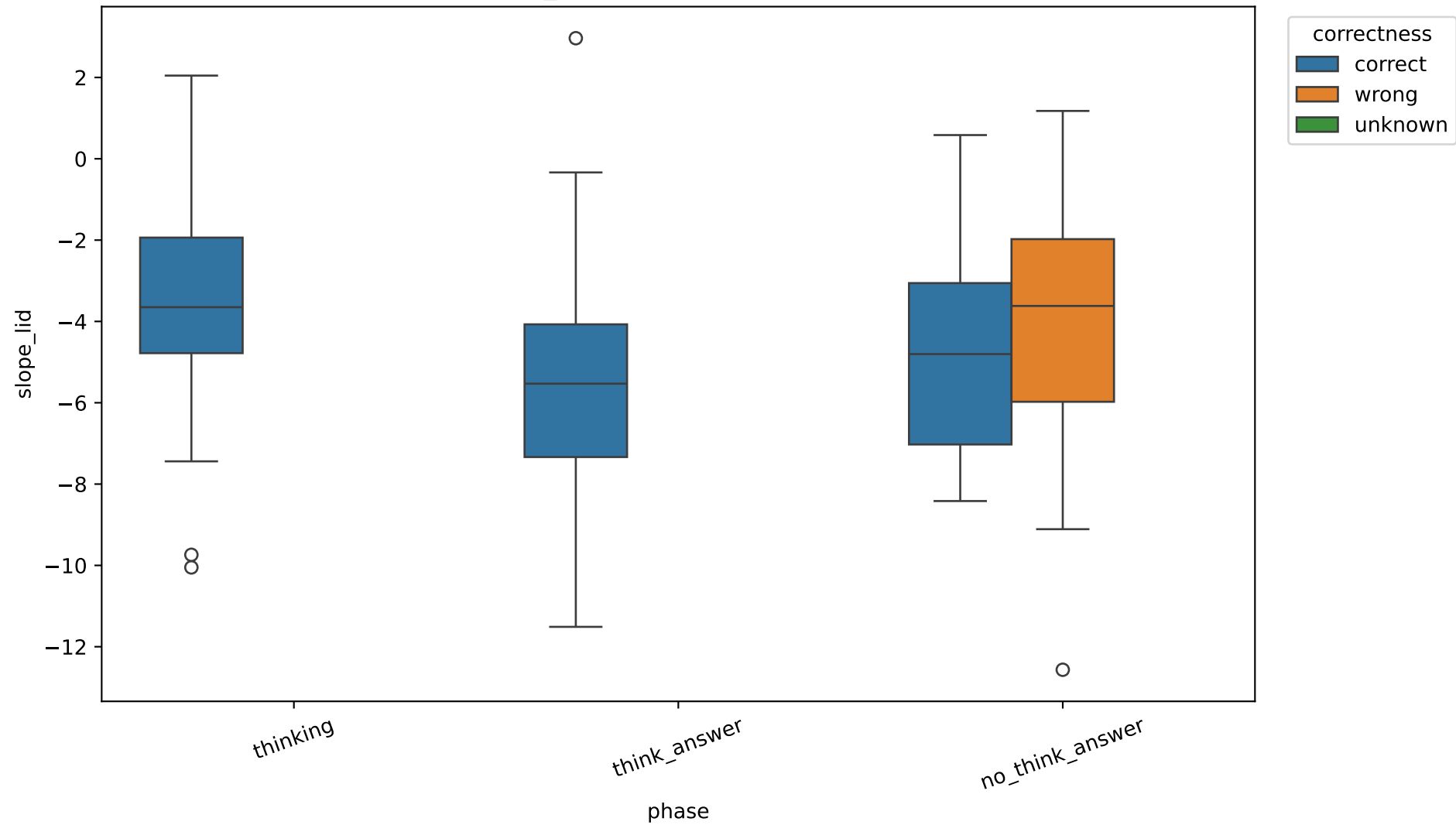
Exp C slope_lid by correctness, 14B, layer 20
