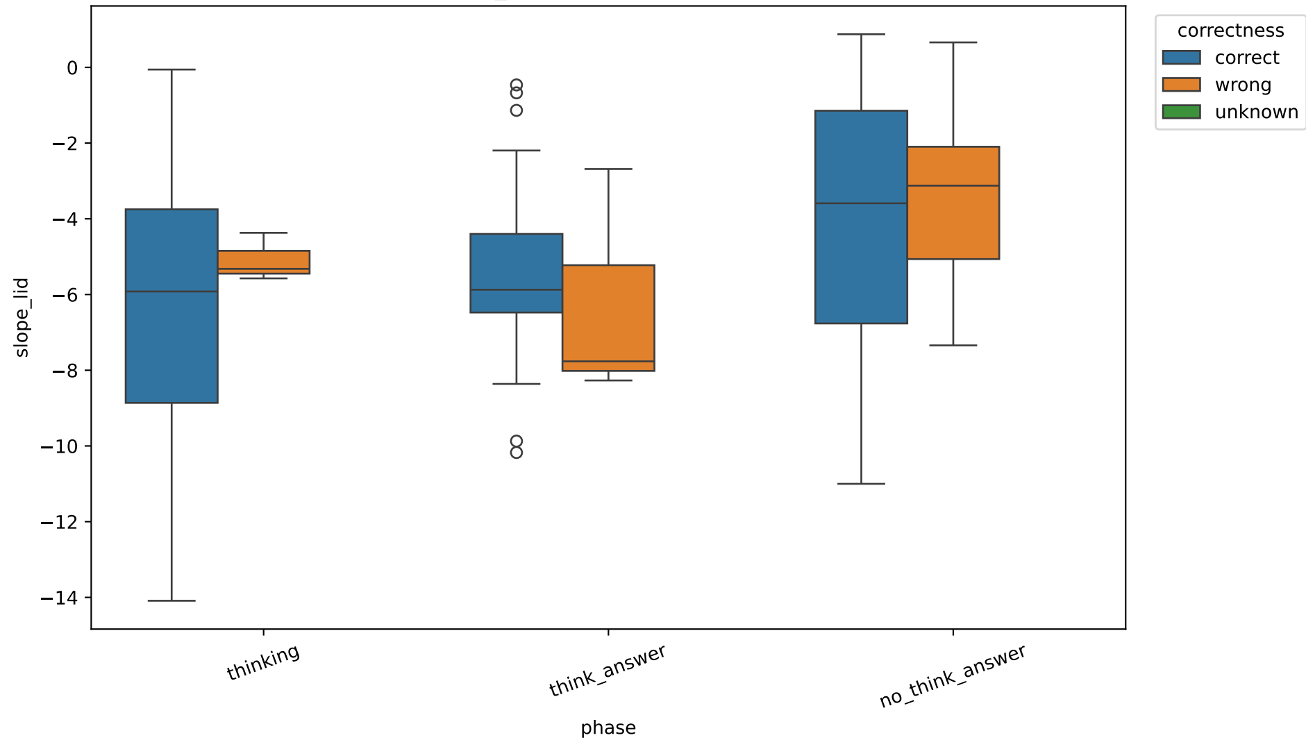
Exp C slope_lid by correctness, 8B, layer 13
