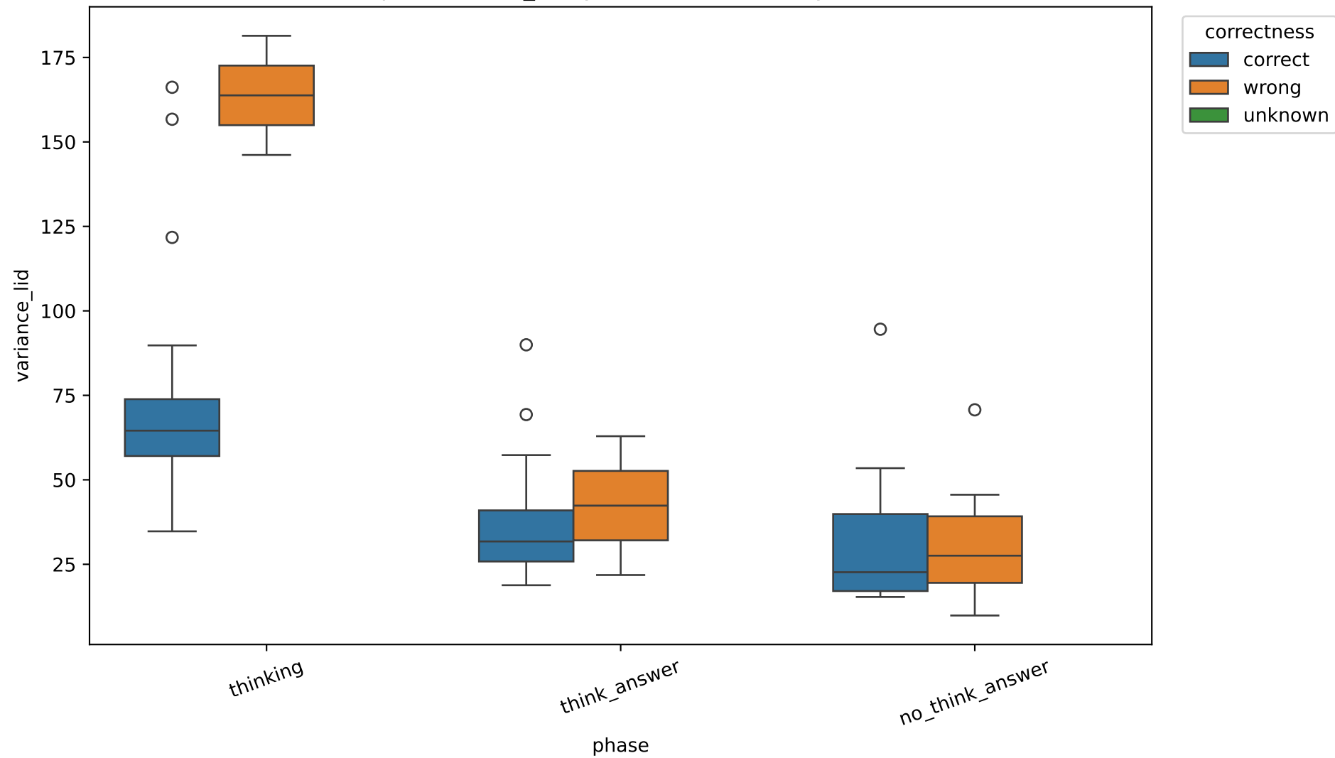
Exp C variance_lid by correctness, 4B, layer 13
