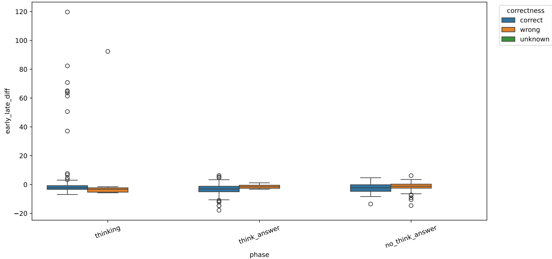
Exp C early_late_diff by correctness, pooled across model sizes, layer 20
