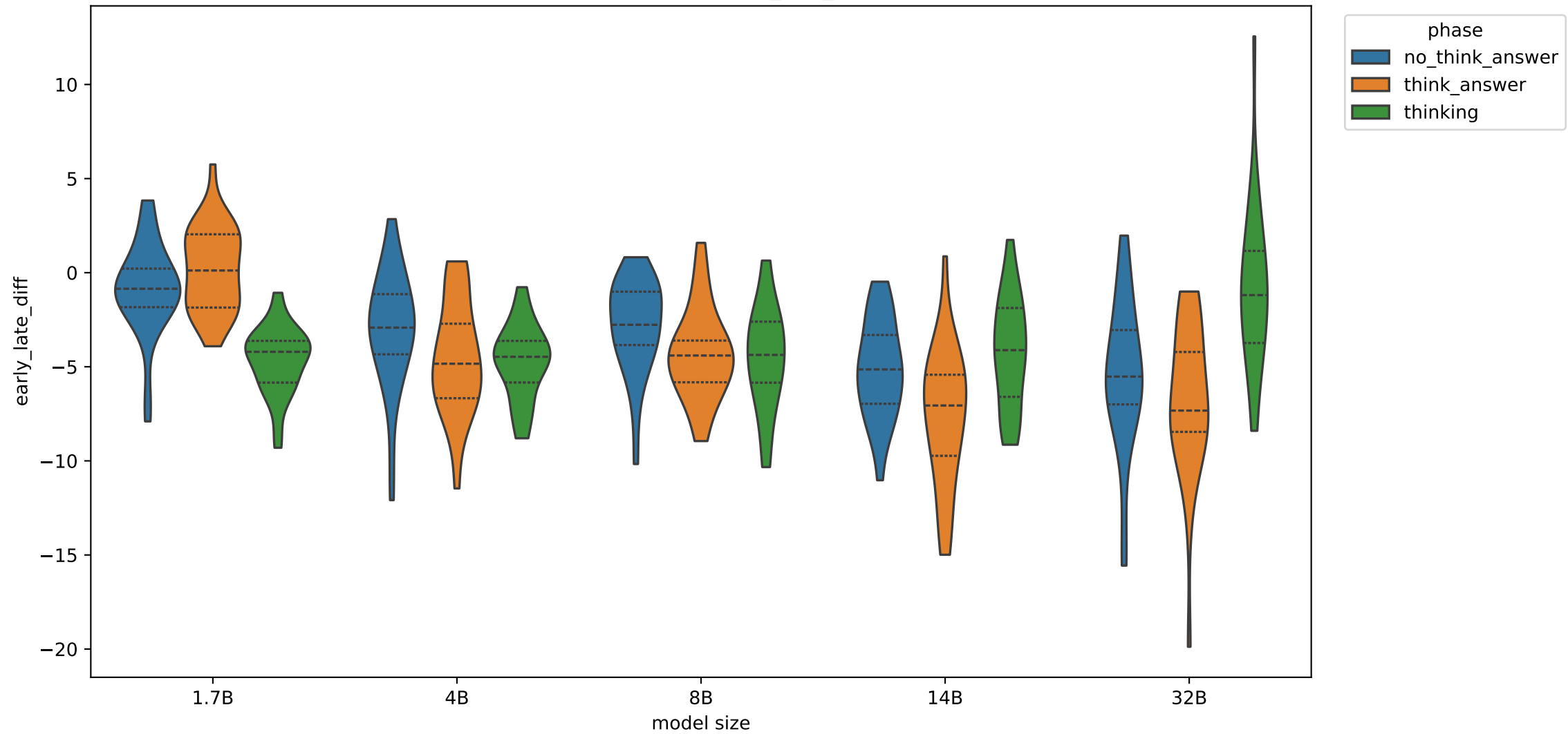
Exp C trajectory statistic: early_late_diff, layer 13
