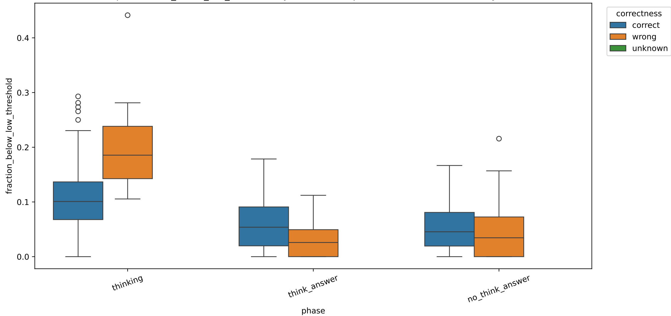
Exp C fraction_below_low_threshold by correctness, pooled across model sizes, layer 20
