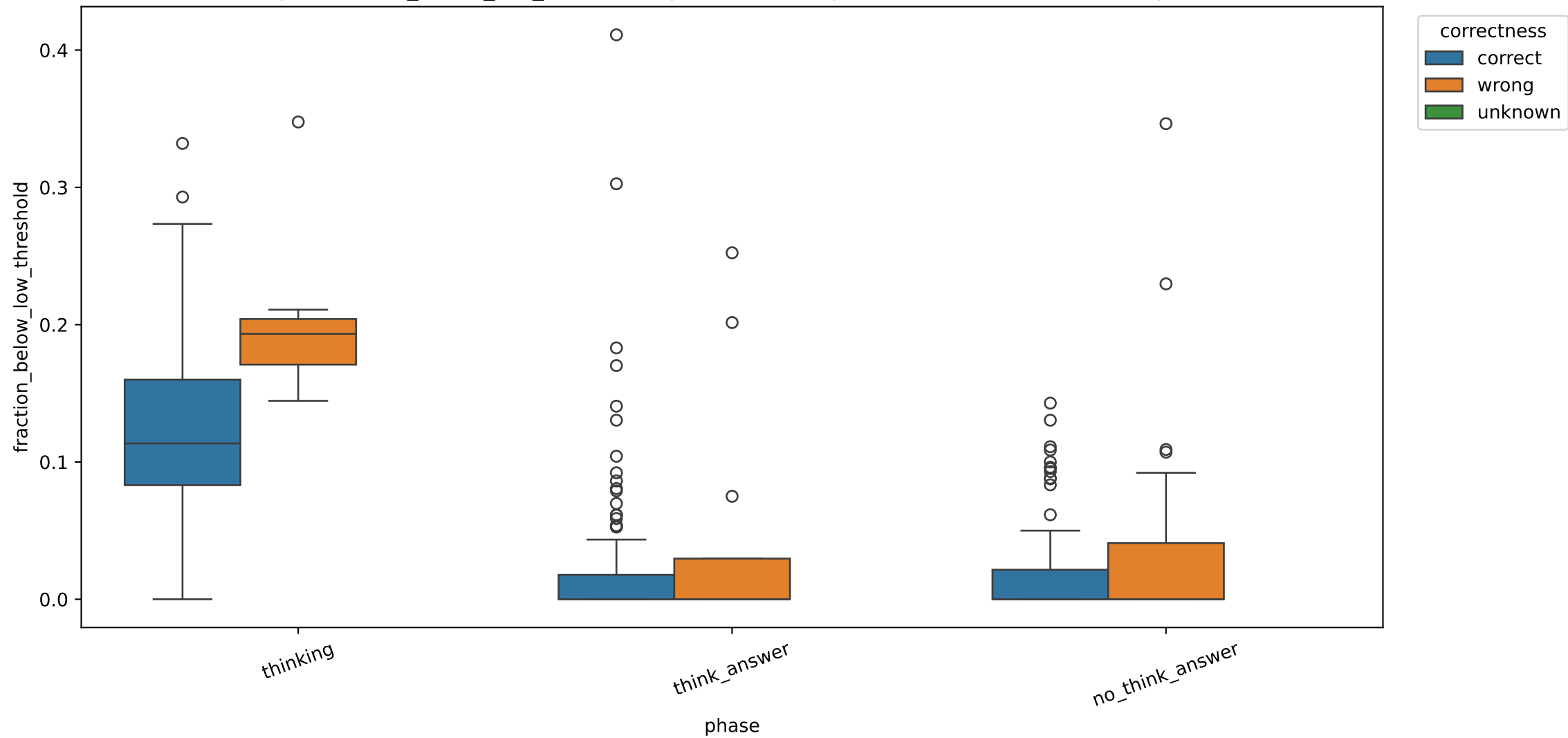
Exp C fraction_below_low_threshold by correctness, pooled across model sizes, layer 6
