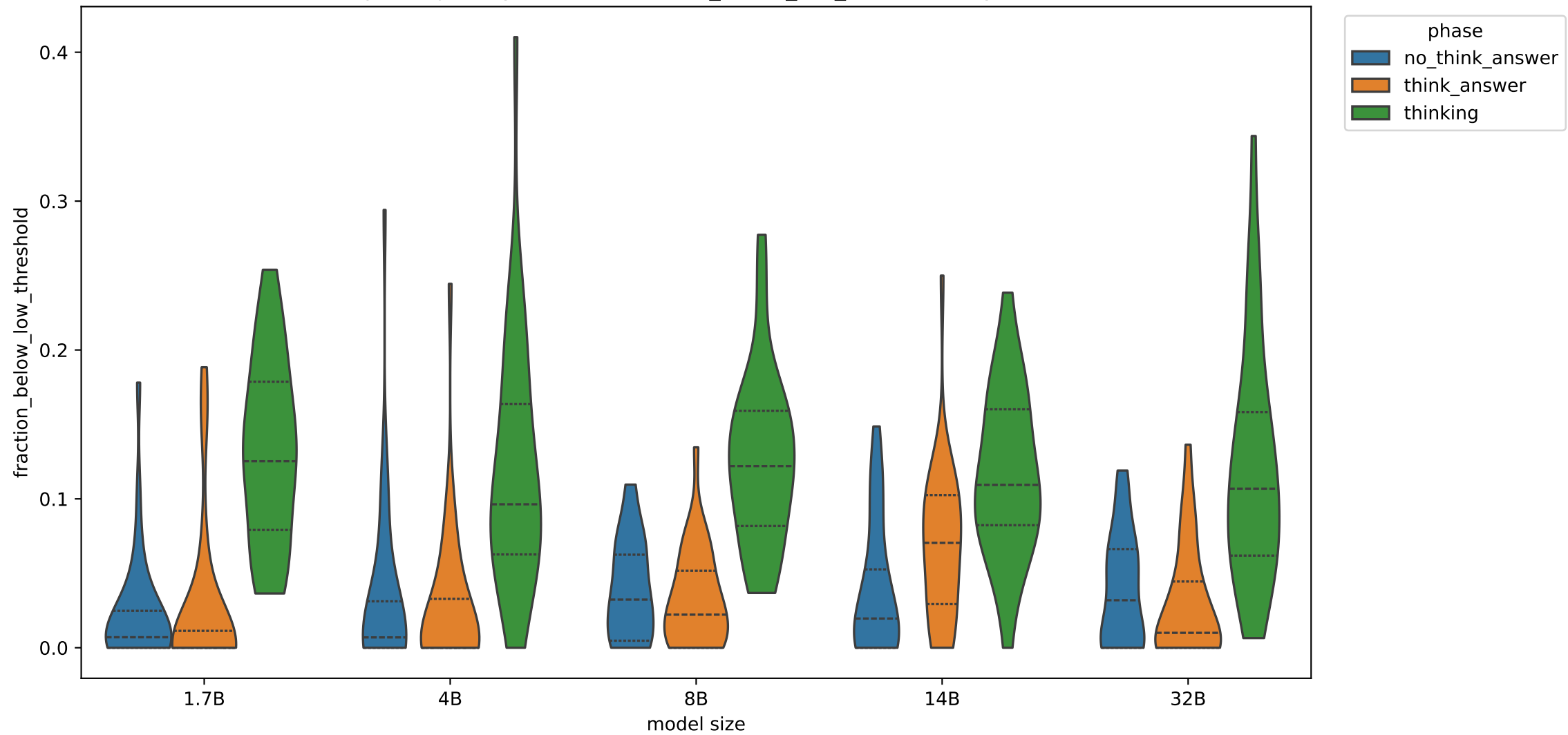
Exp C trajectory statistic: fraction_below_low_threshold, layer 13
