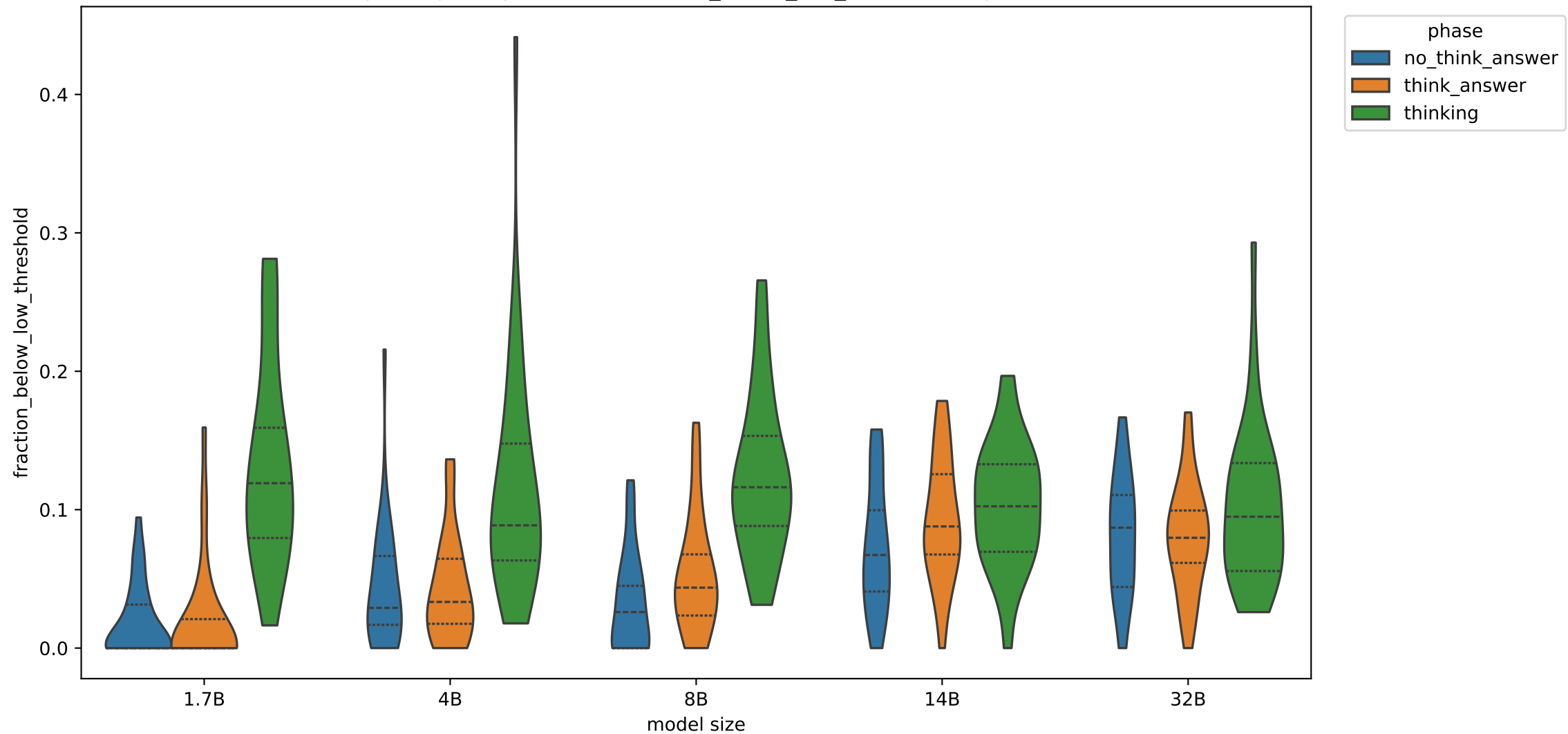
Exp C trajectory statistic: fraction_below_low_threshold, layer 20
