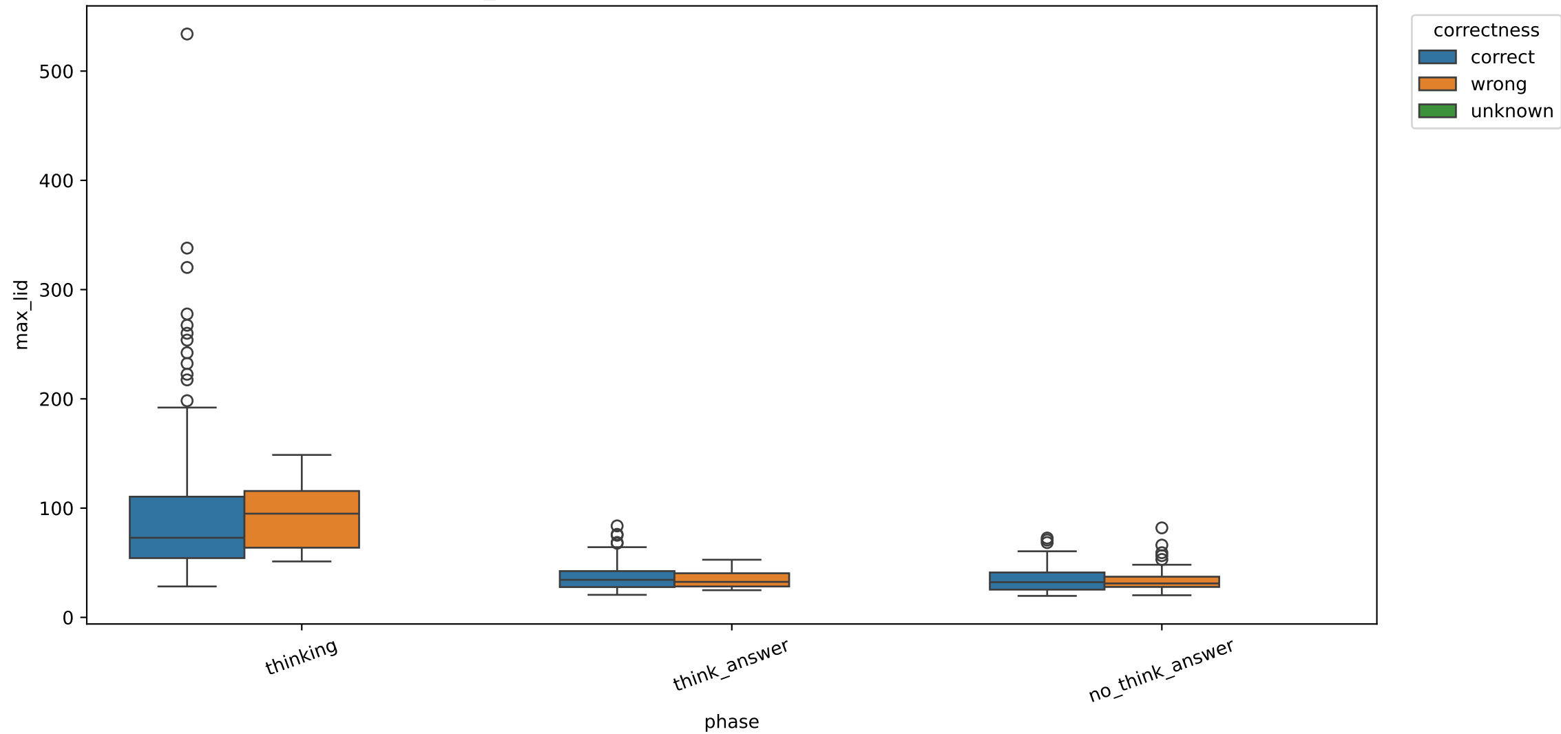
Exp C max_lid by correctness, pooled across model sizes, layer 13
