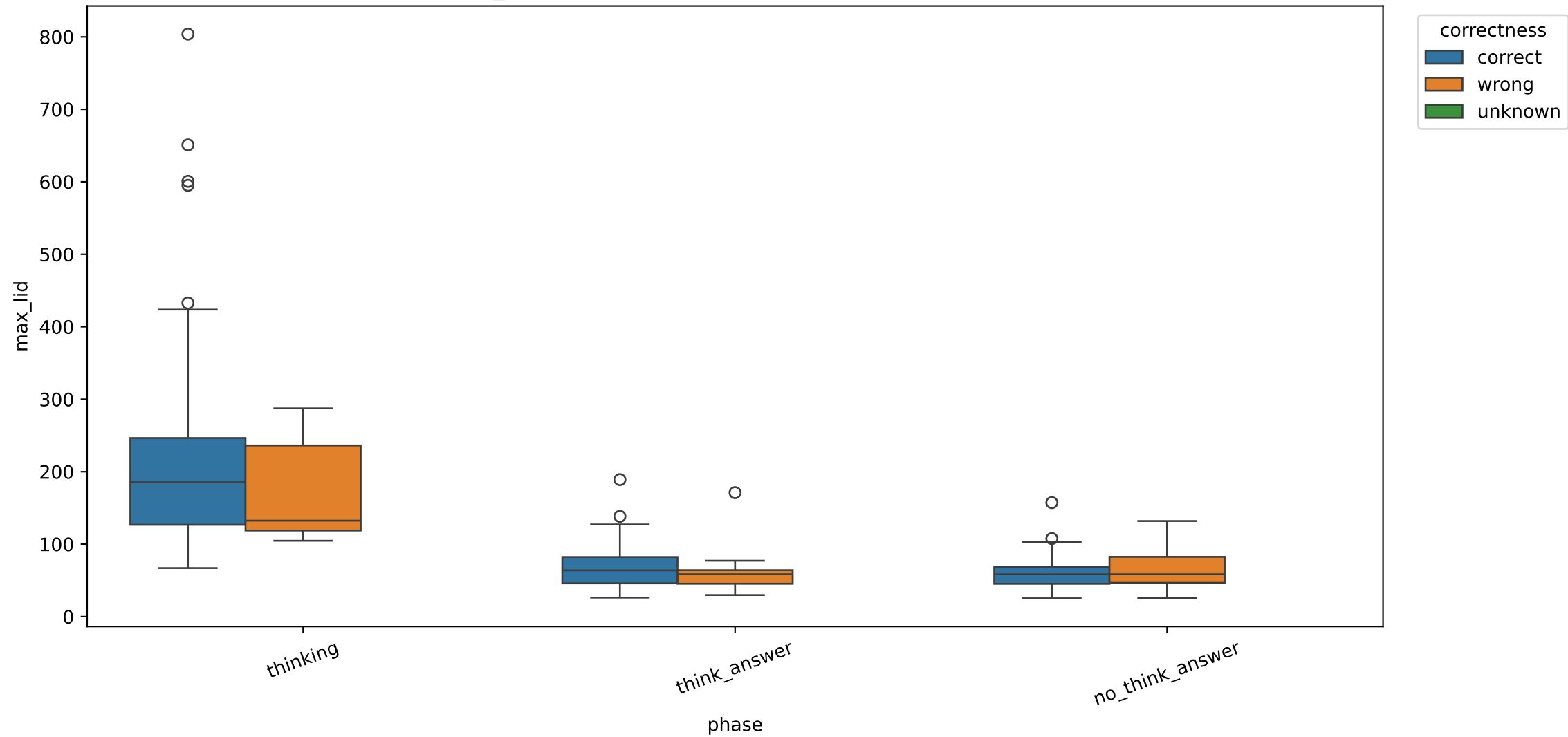
Exp C max_lid by correctness, pooled across model sizes, layer 6
