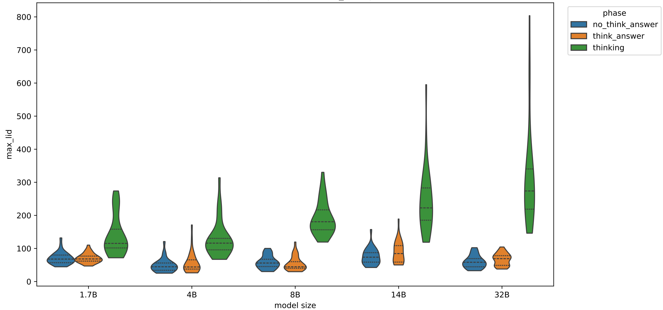
Exp C trajectory statistic: max_lid, layer 6
