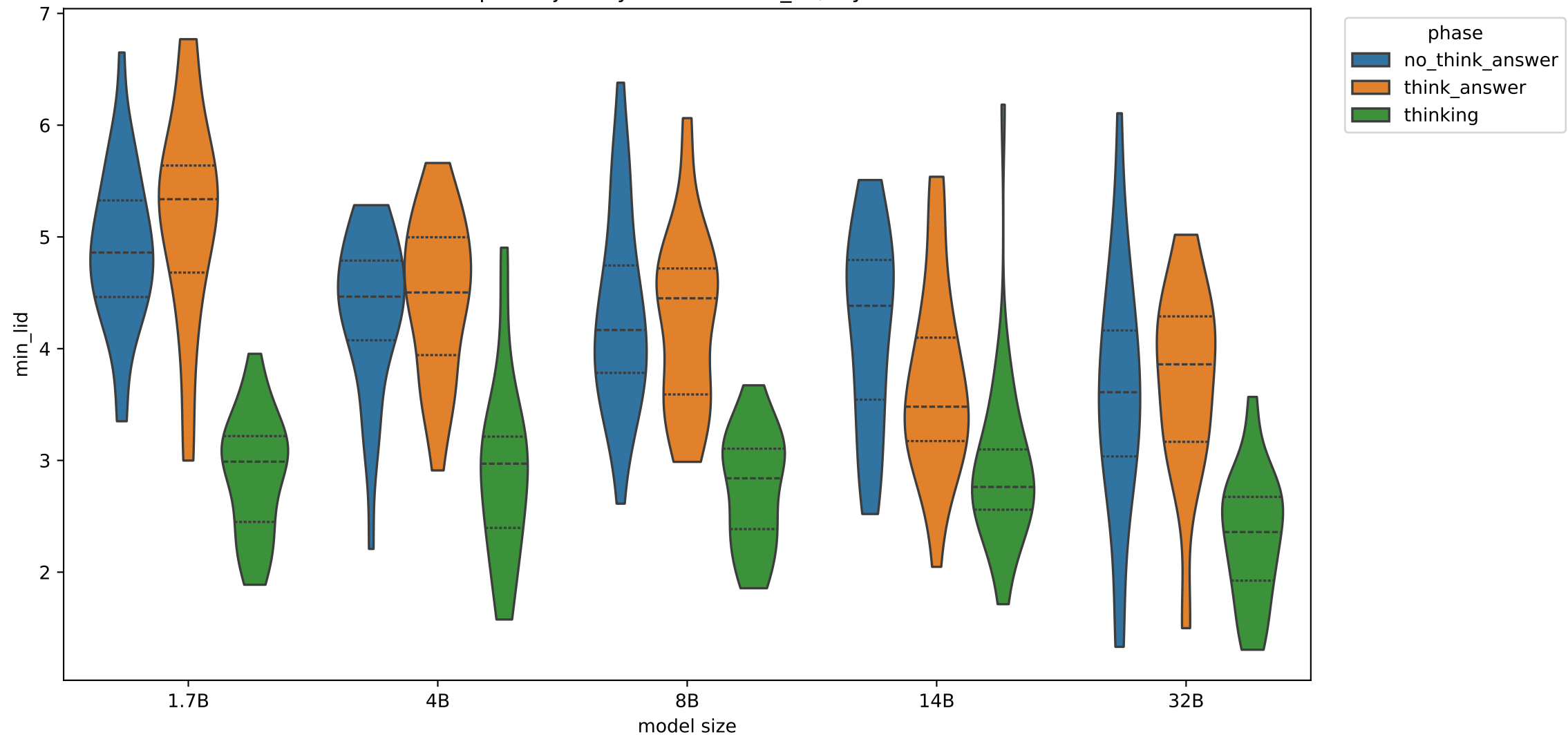
Exp C trajectory statistic: min_lid, layer 13
