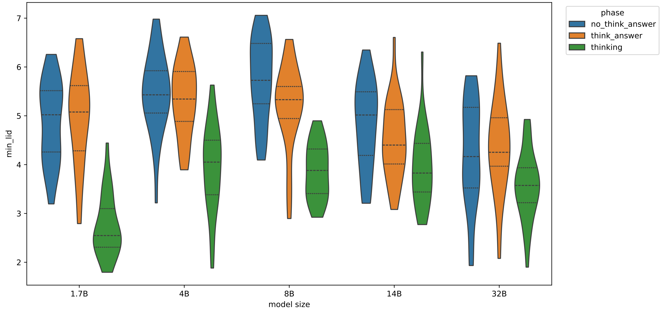
Exp C trajectory statistic: min_lid, layer 20
