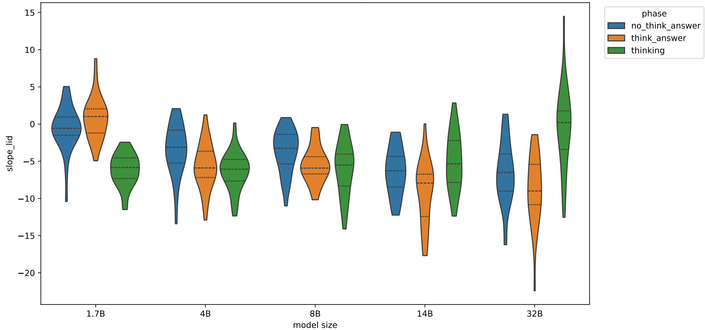
Exp C trajectory statistic: slope_lid, layer 13
