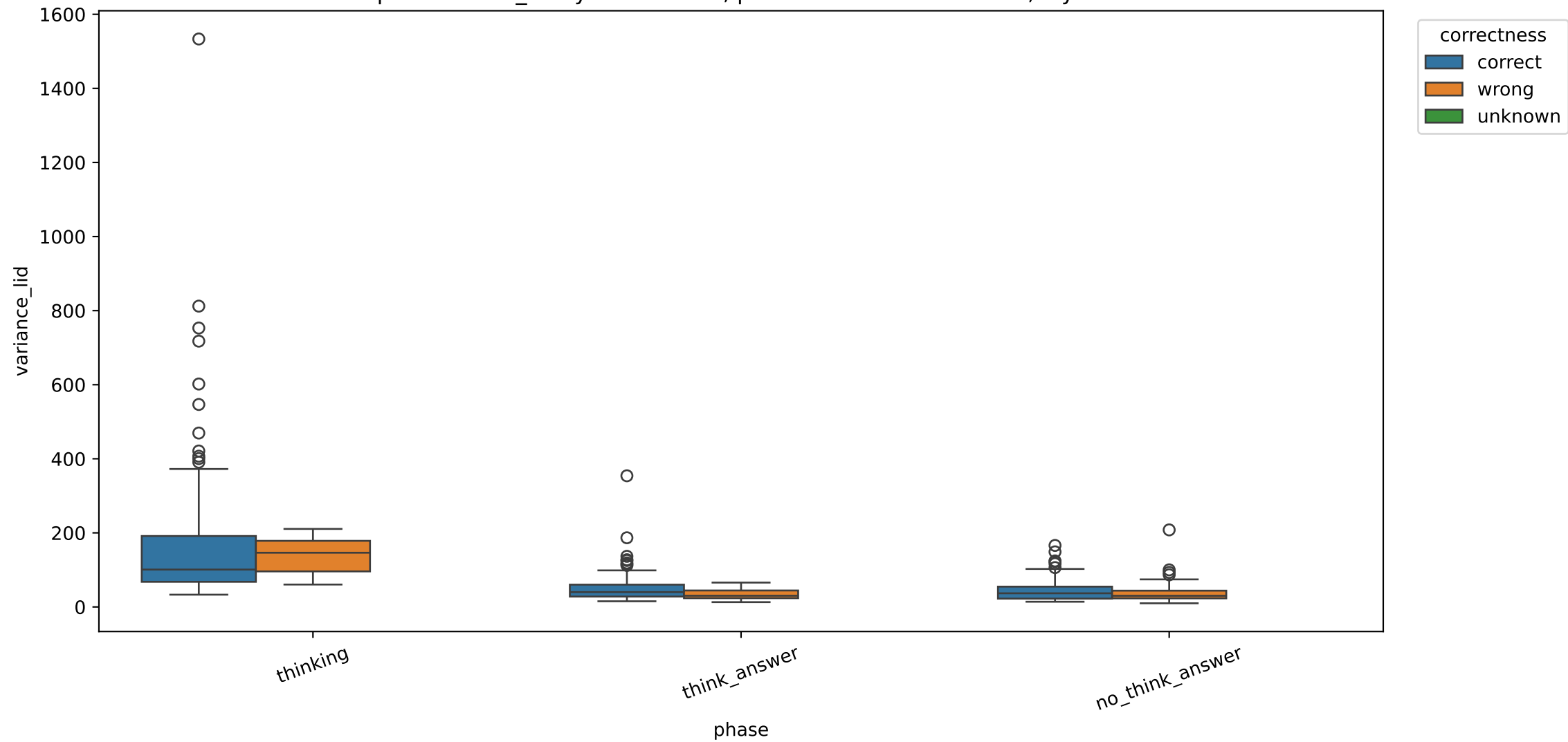
Exp C variance_lid by correctness, pooled across model sizes, layer 13
