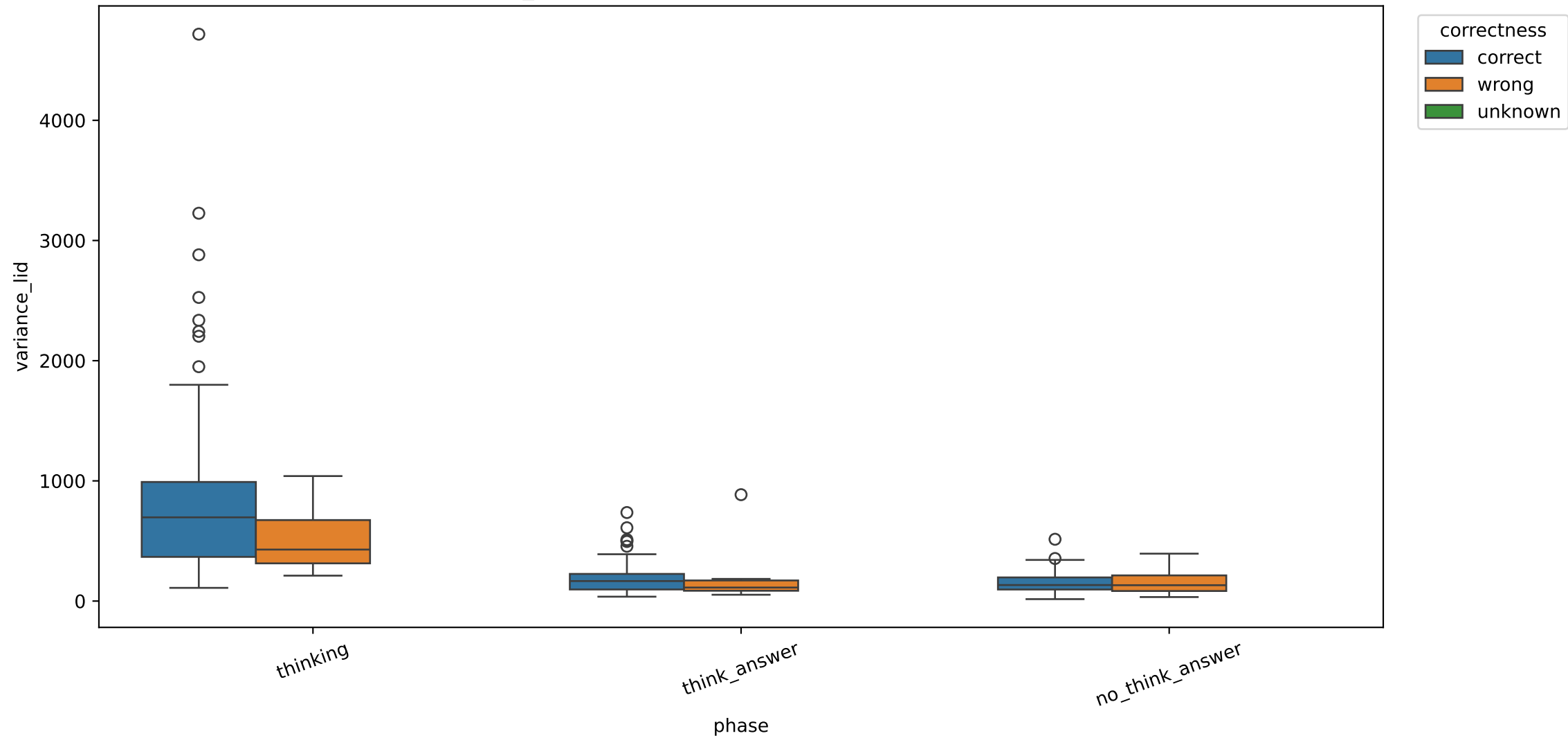
Exp C variance_lid by correctness, pooled across model sizes, layer 6
