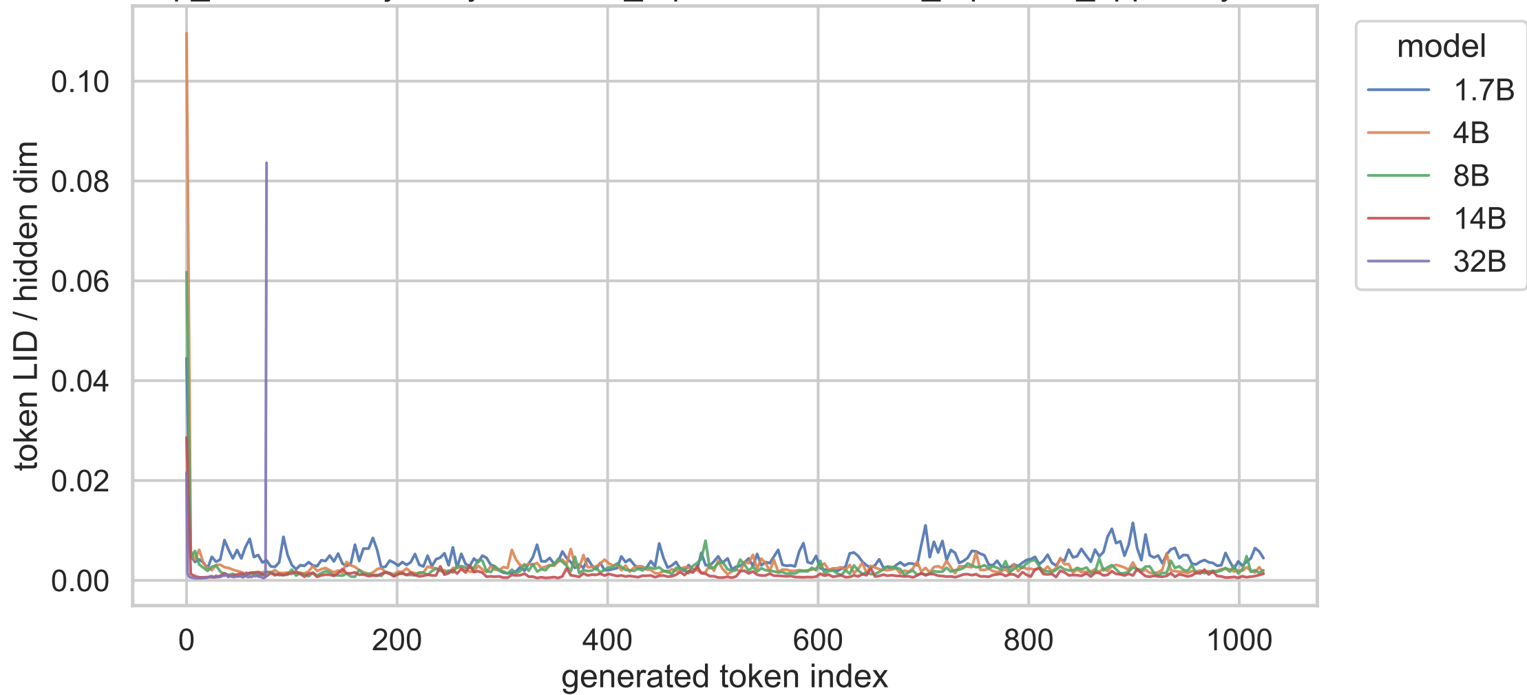
exp_a shared trajectory, constant_repetition, constant_repetition_apple, layer 13
