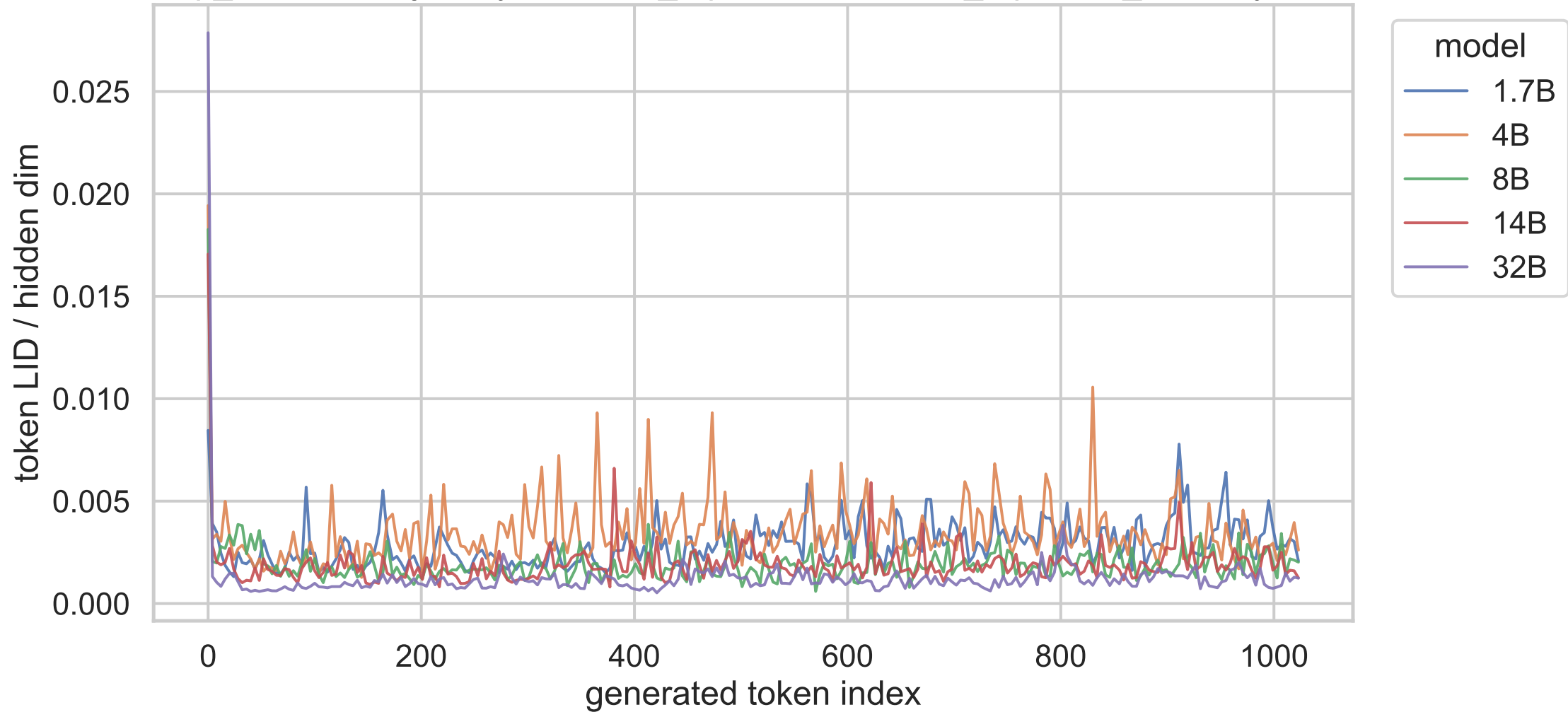
exp_a shared trajectory, constant_repetition, constant_repetition_data, layer 20
