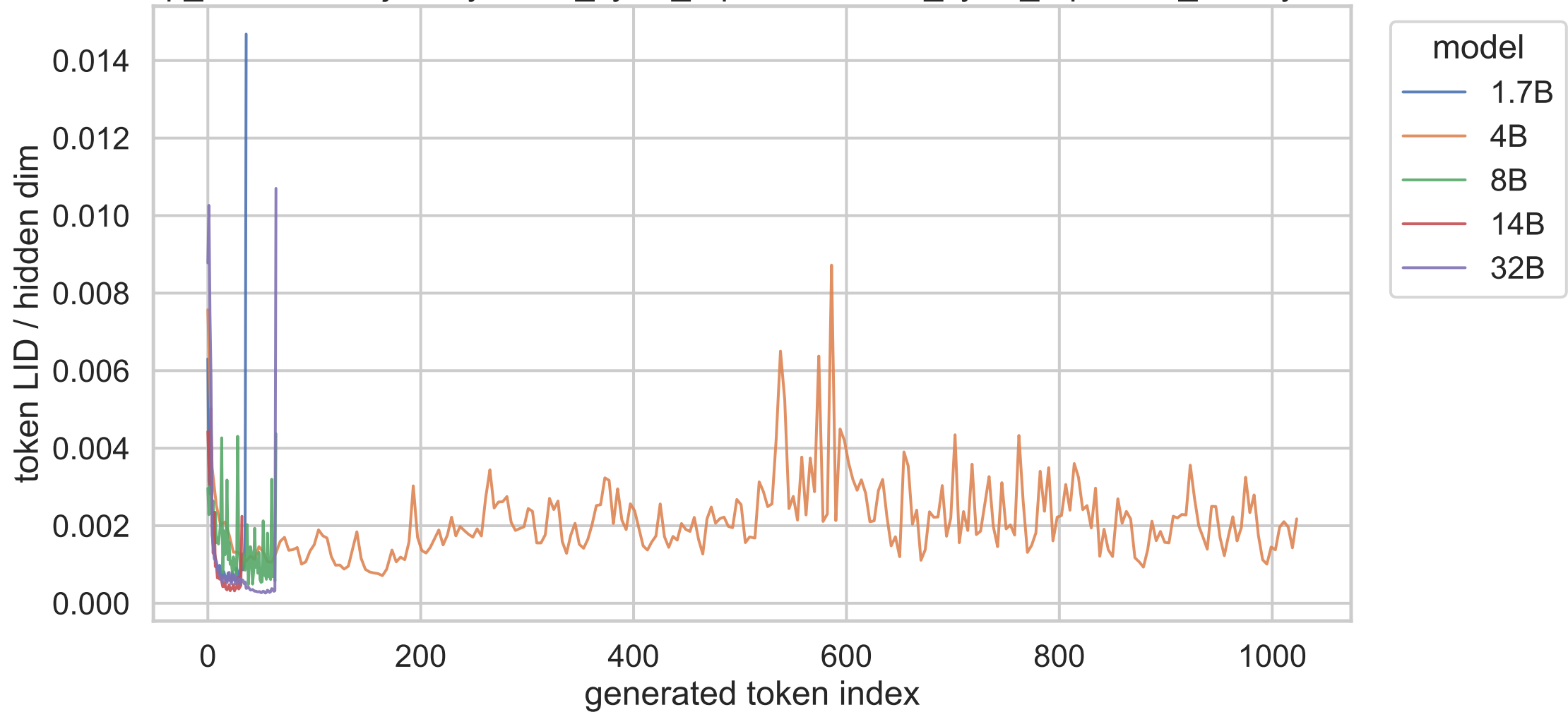
exp_a shared trajectory, short_cycle_repetition, short_cycle_repetition_02, layer 20
