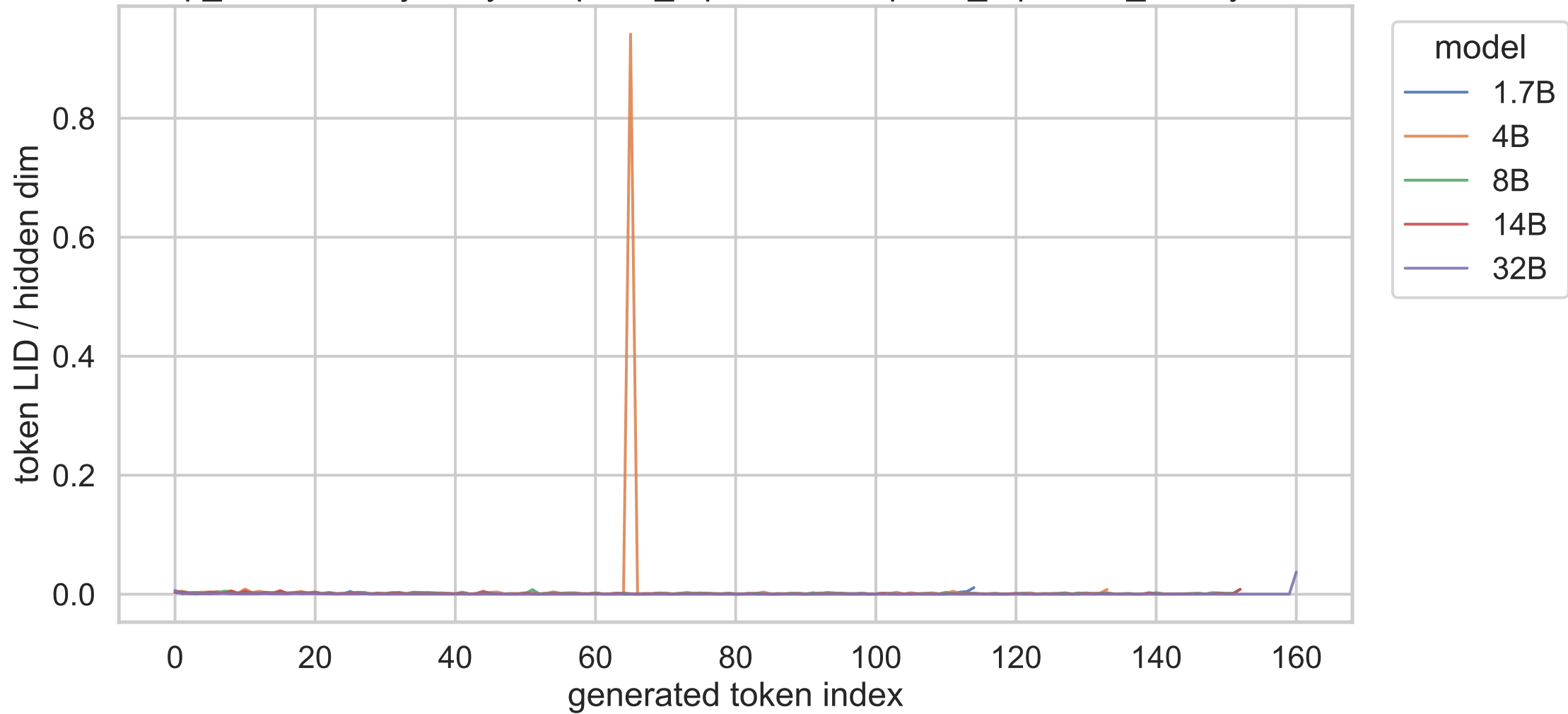
exp_a shared trajectory, templatic_repetition, templatic_repetition_03, layer 20
