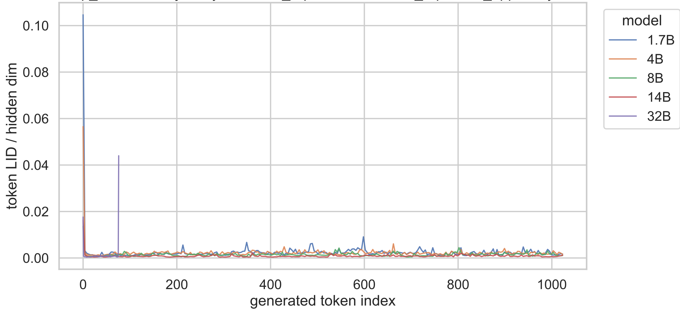
exp_a shared trajectory, constant_repetition, constant_repetition_apple, layer 6
