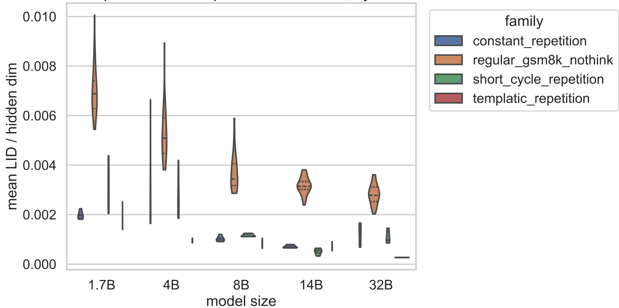
Exp A mean full-output LID distributions, layer 6
