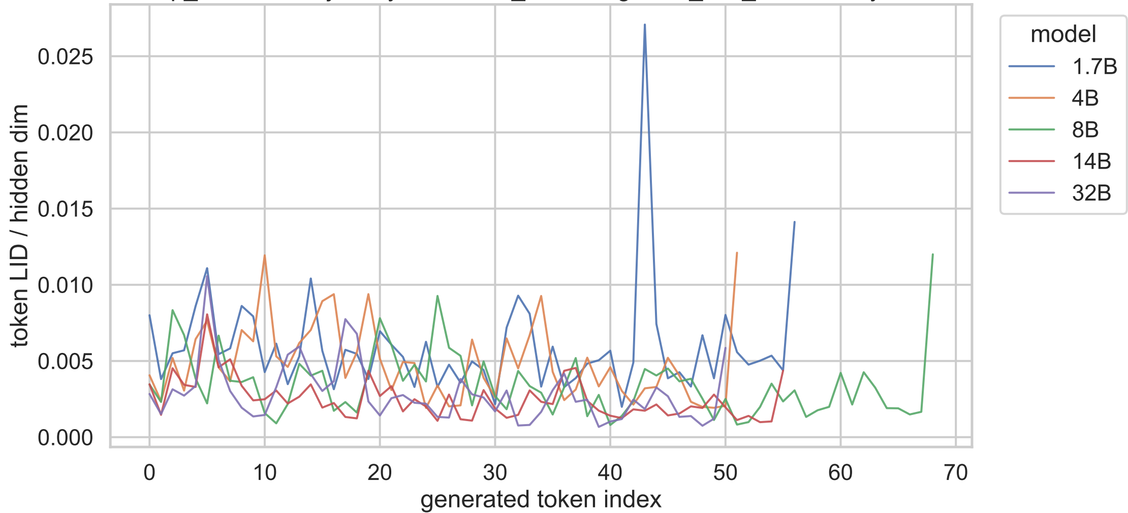
exp_b shared trajectory, irrelevant_context, gsm8k_test_000052, layer 13
