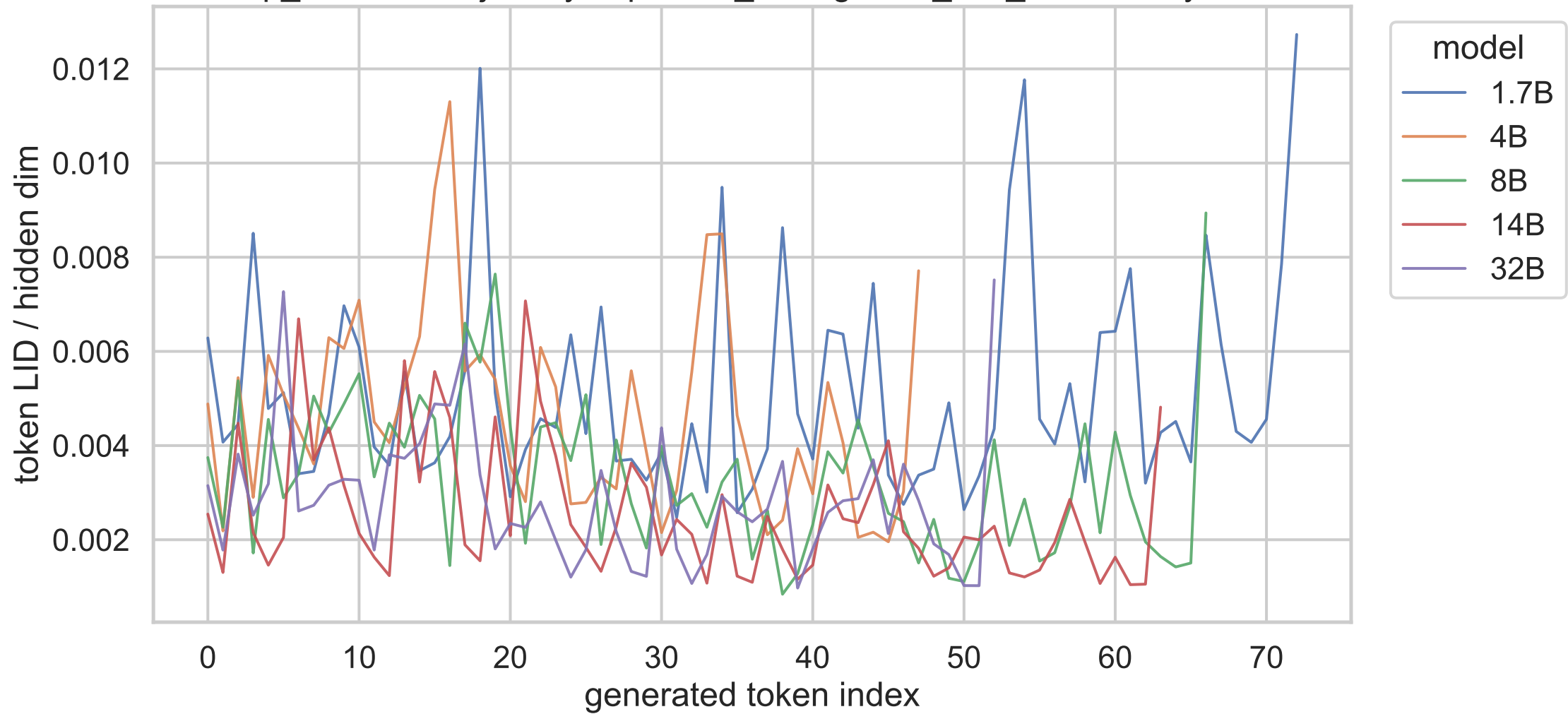
exp_b shared trajectory, repetitive_filler, gsm8k_test_000052, layer 13
