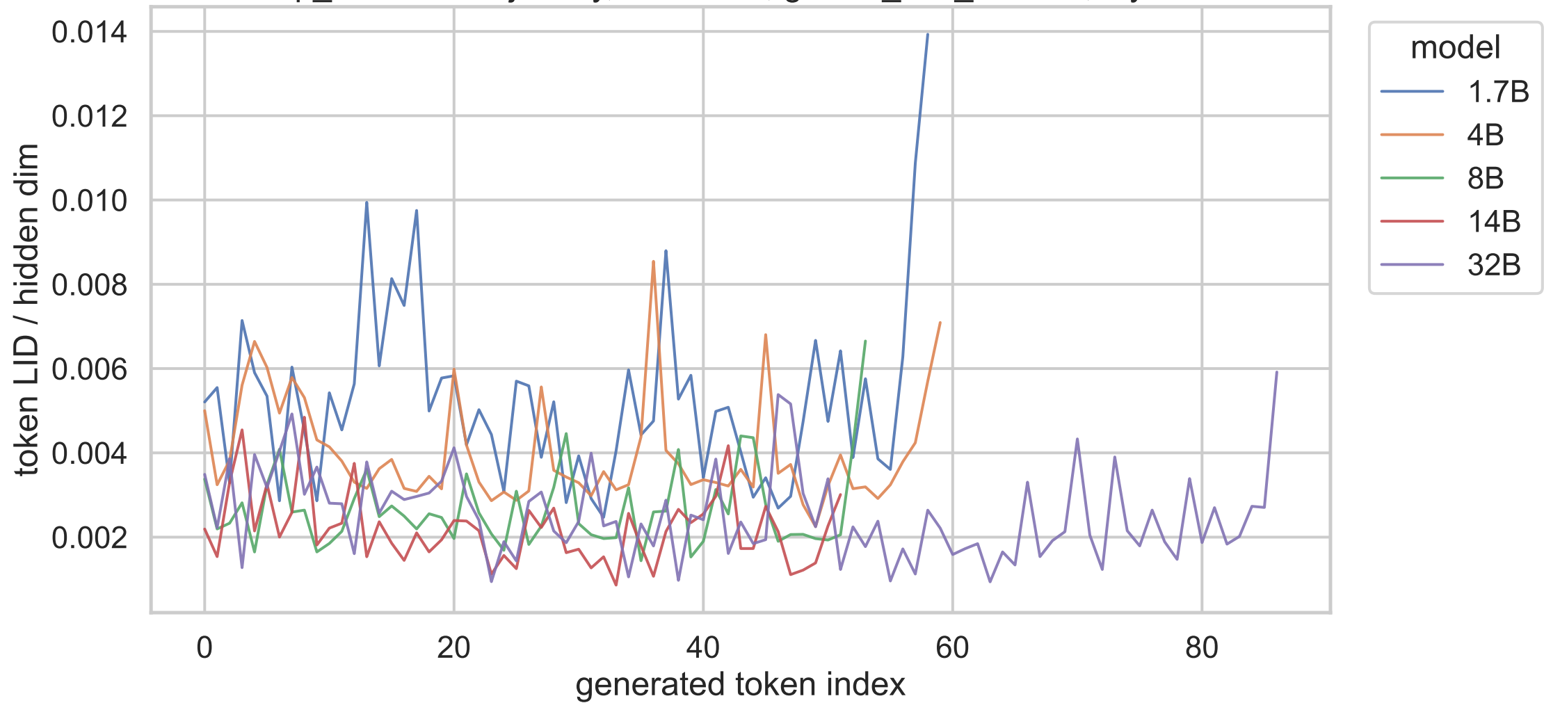
exp_b shared trajectory, canonical, gsm8k_test_000010, layer 20
