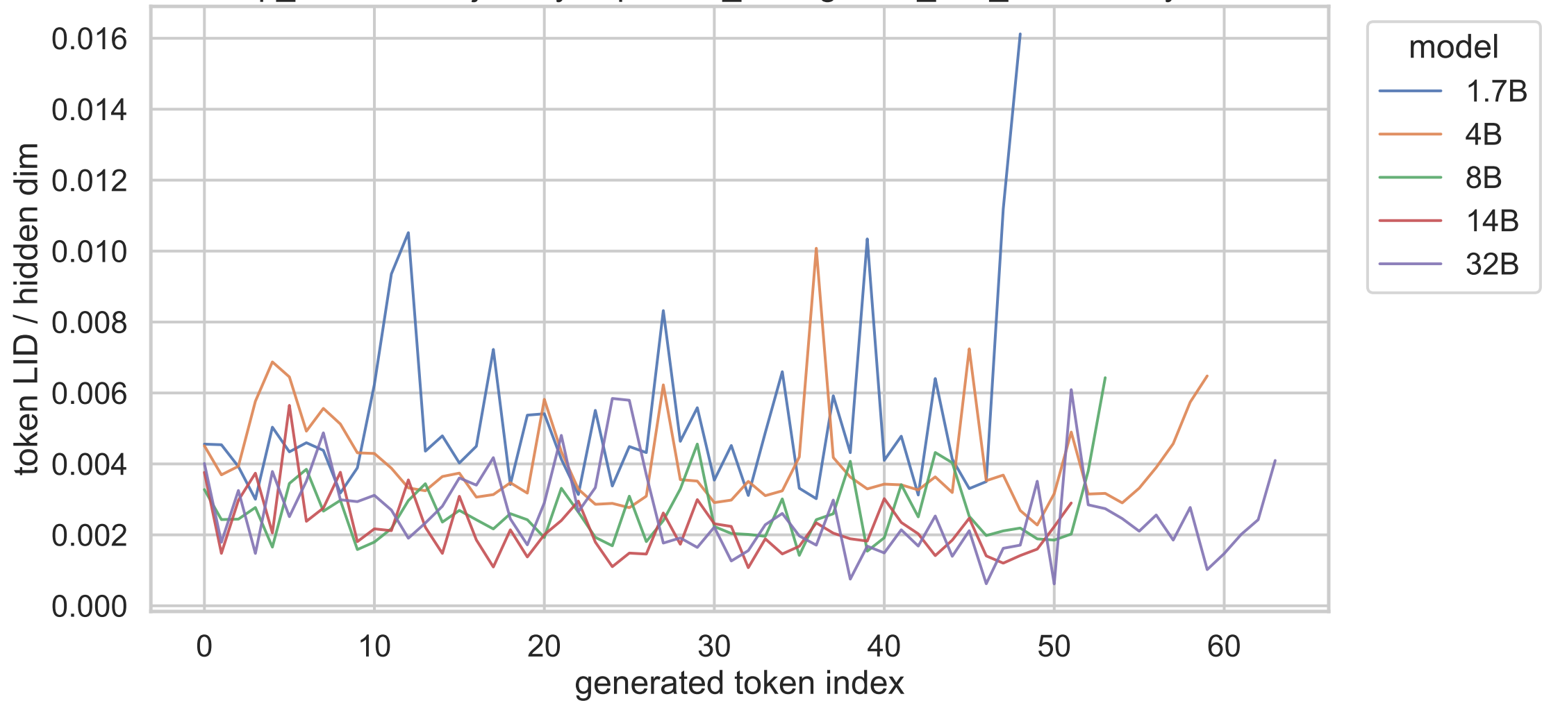
exp_b shared trajectory, repetitive_filler, gsm8k_test_000010, layer 20
