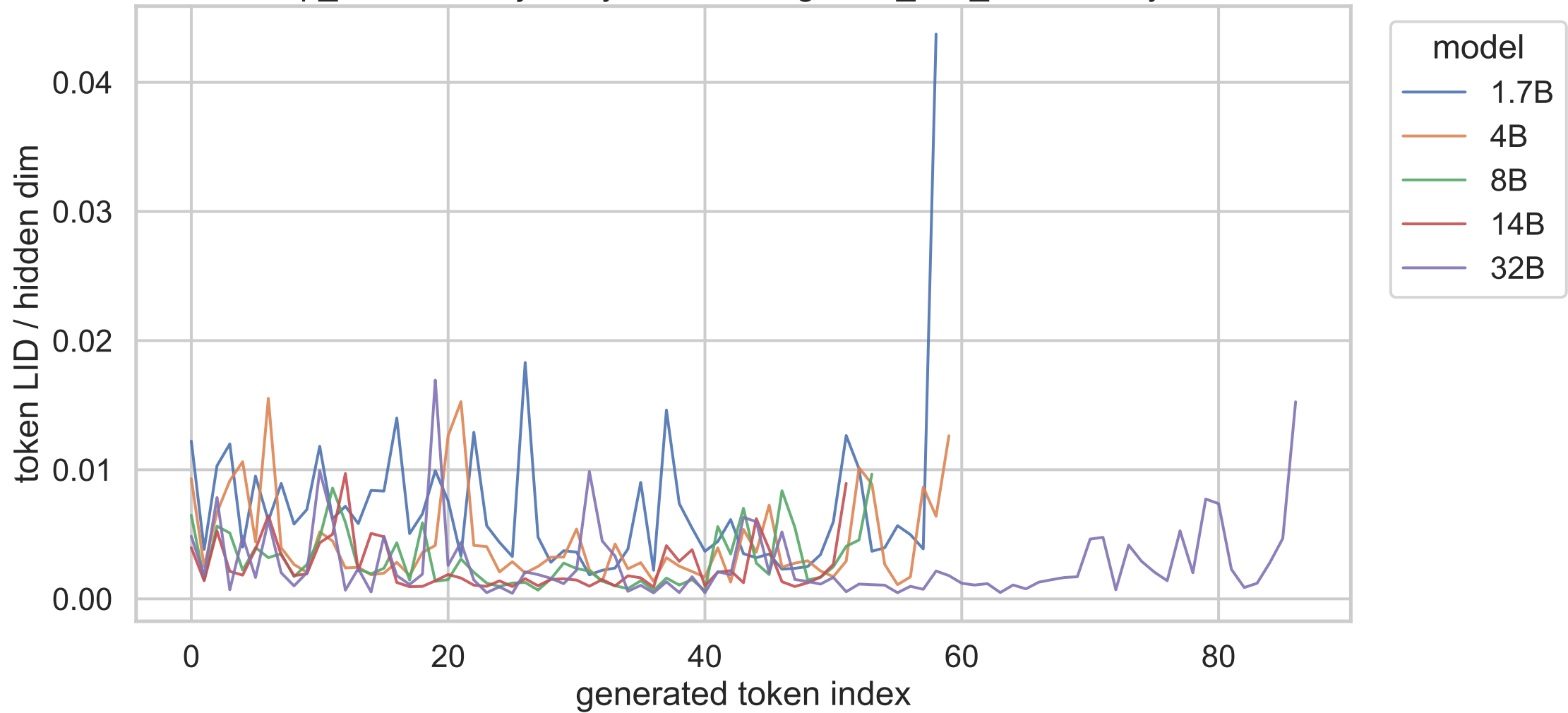
exp_b shared trajectory, canonical, gsm8k_test_000010, layer 6
