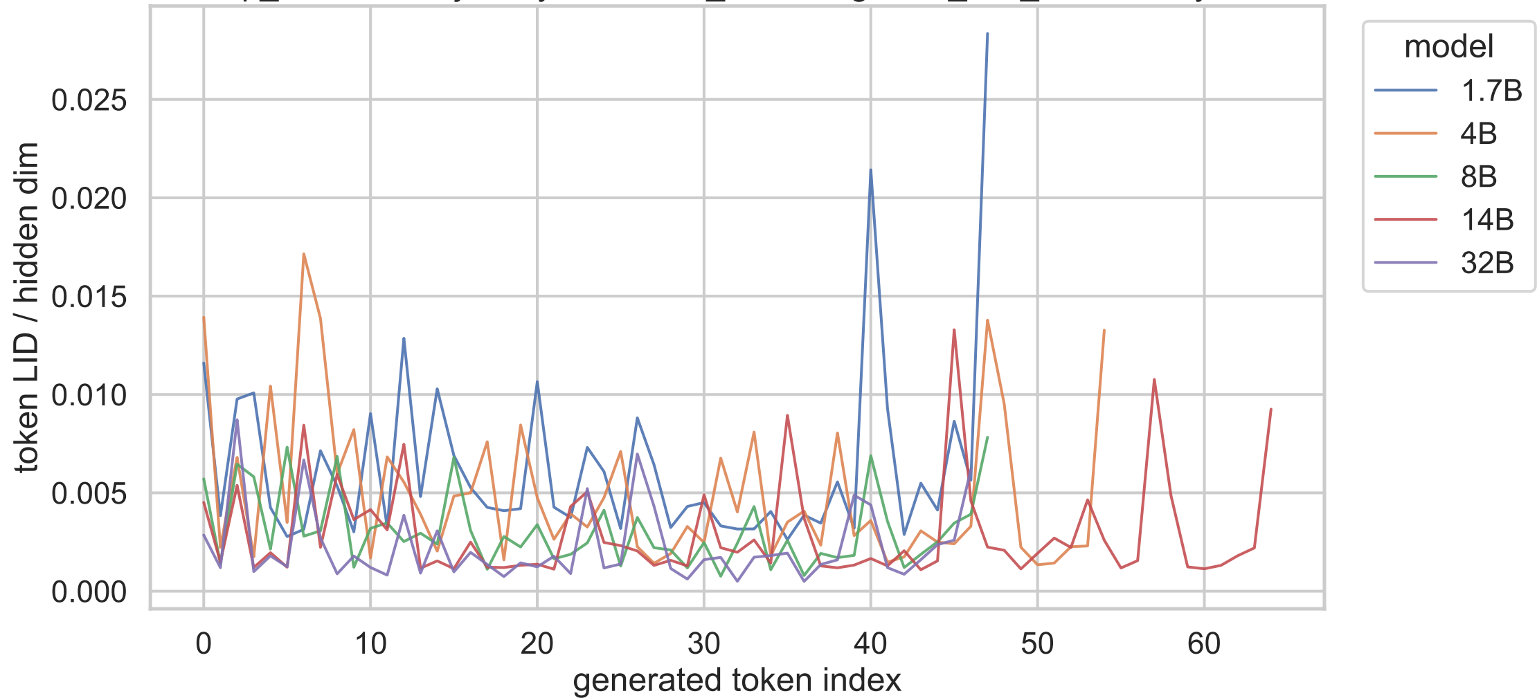
exp_b shared trajectory, irrelevant_context, gsm8k_test_000003, layer 6
