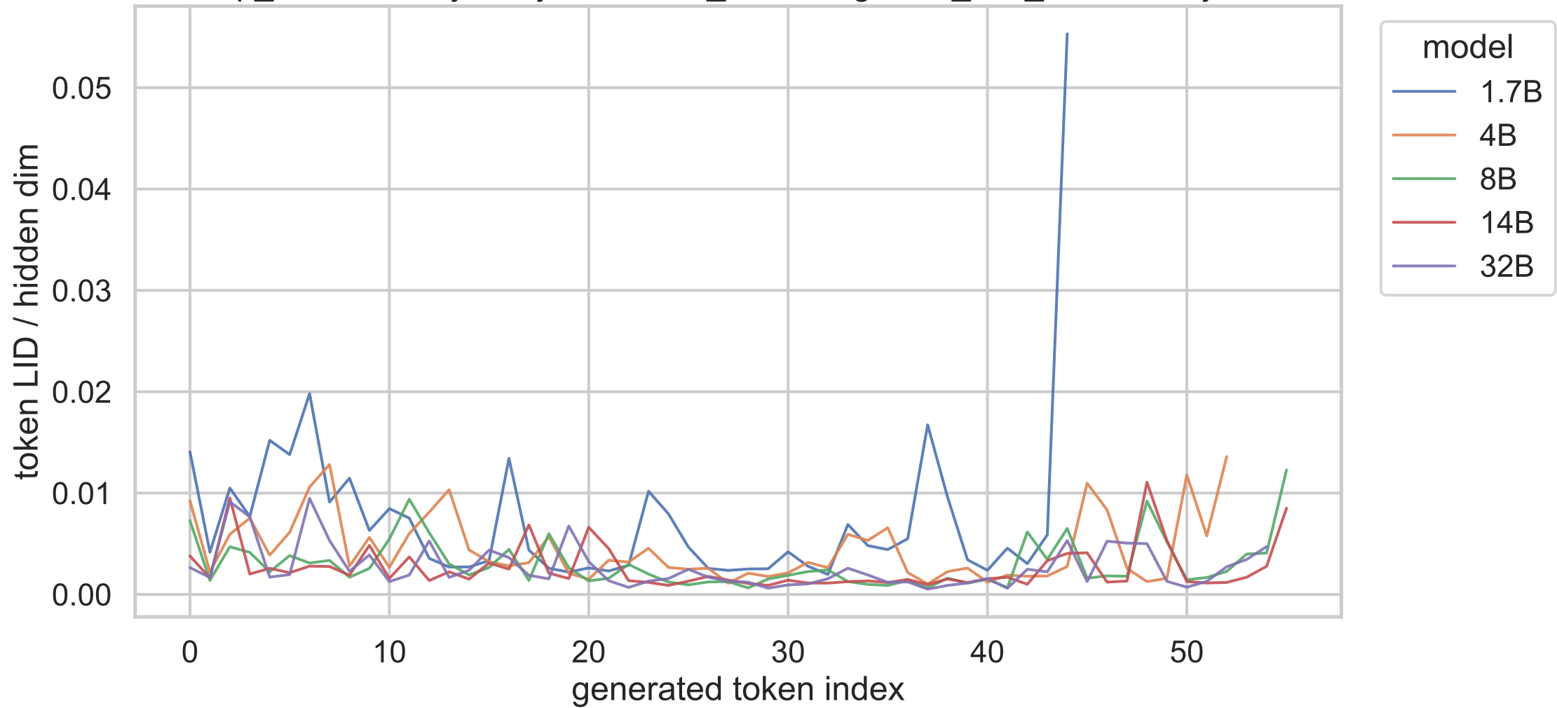
exp_b shared trajectory, irrelevant_context, gsm8k_test_000010, layer 6
