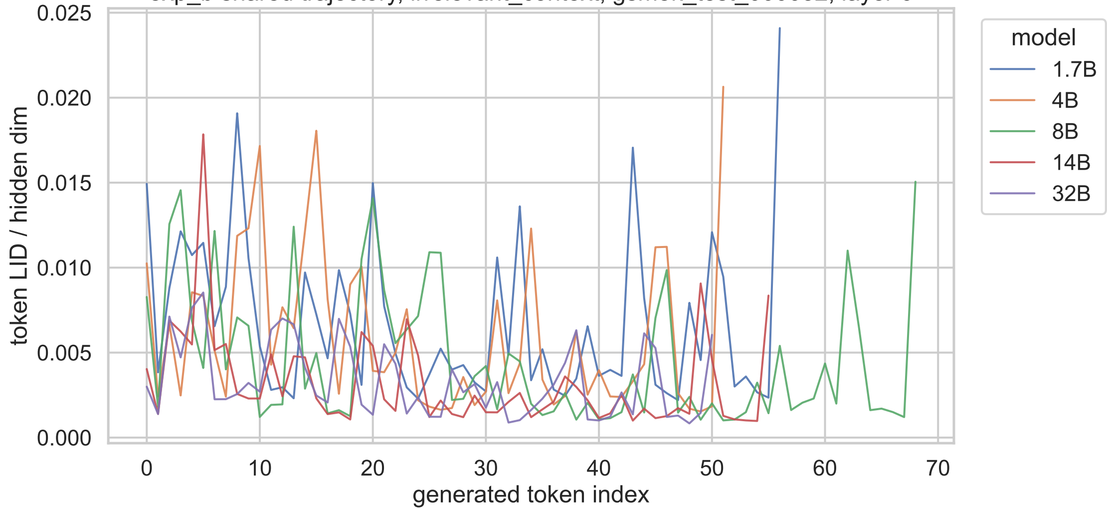
exp_b shared trajectory, irrelevant_context, gsm8k_test_000052, layer 6
