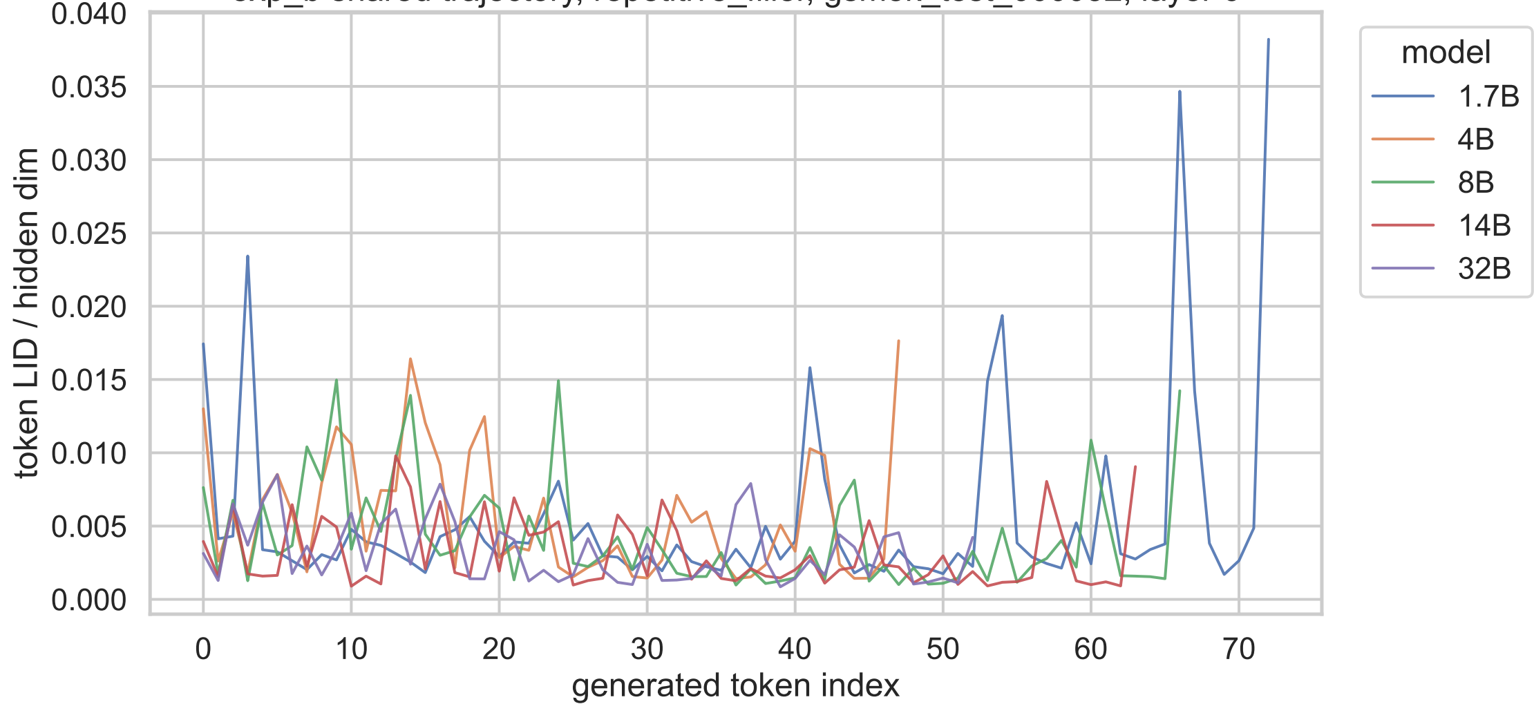
exp_b shared trajectory, repetitive_filler, gsm8k_test_000052, layer 6
