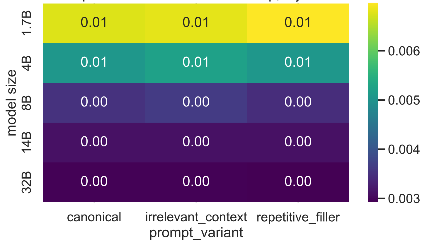
Exp B mean answer LID heatmap, layer 6
