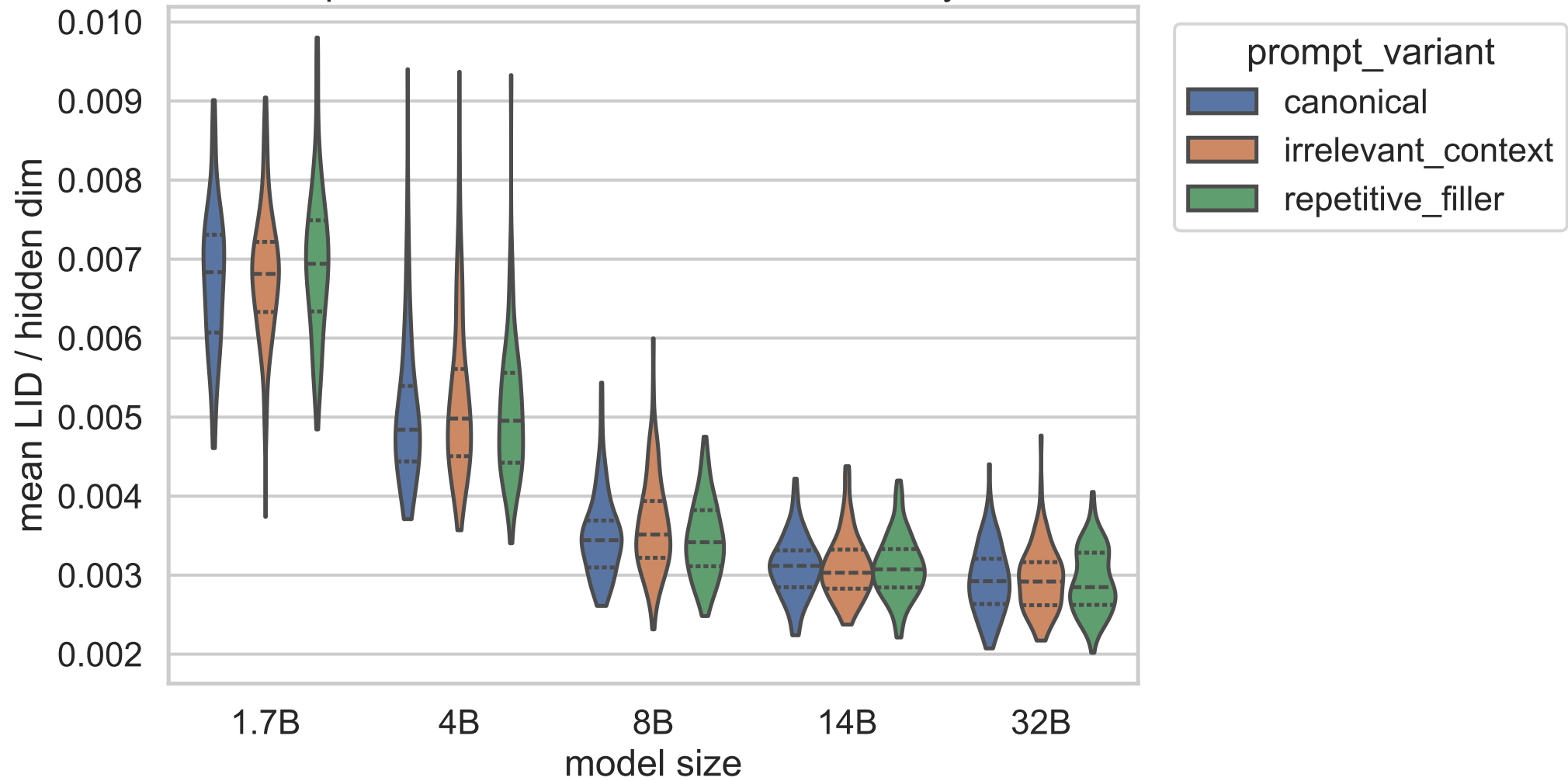
Exp B mean answer LID distributions, layer 6
