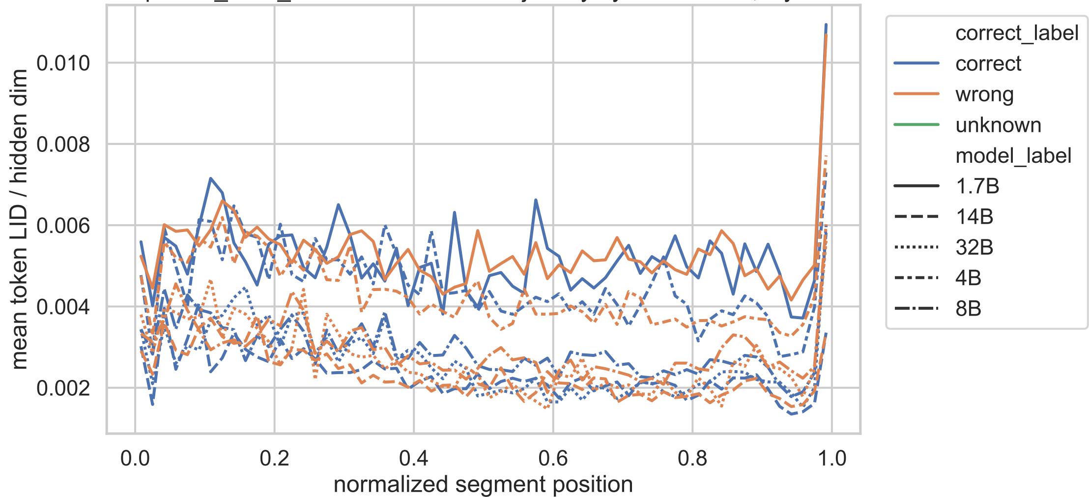
Exp C no_think_answer normalized trajectory by correctness, layer 13
