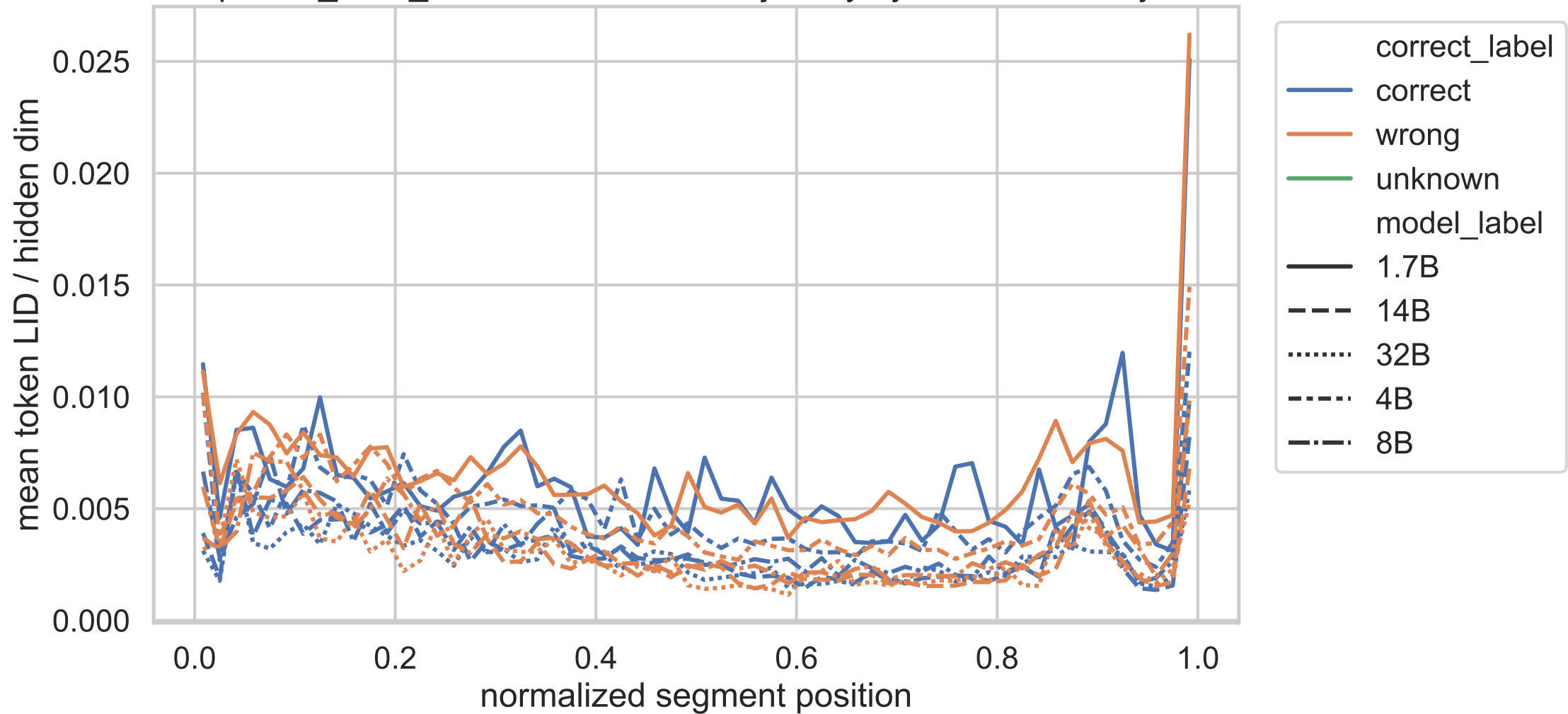
Exp C no_think_answer normalized trajectory by correctness, layer 6
