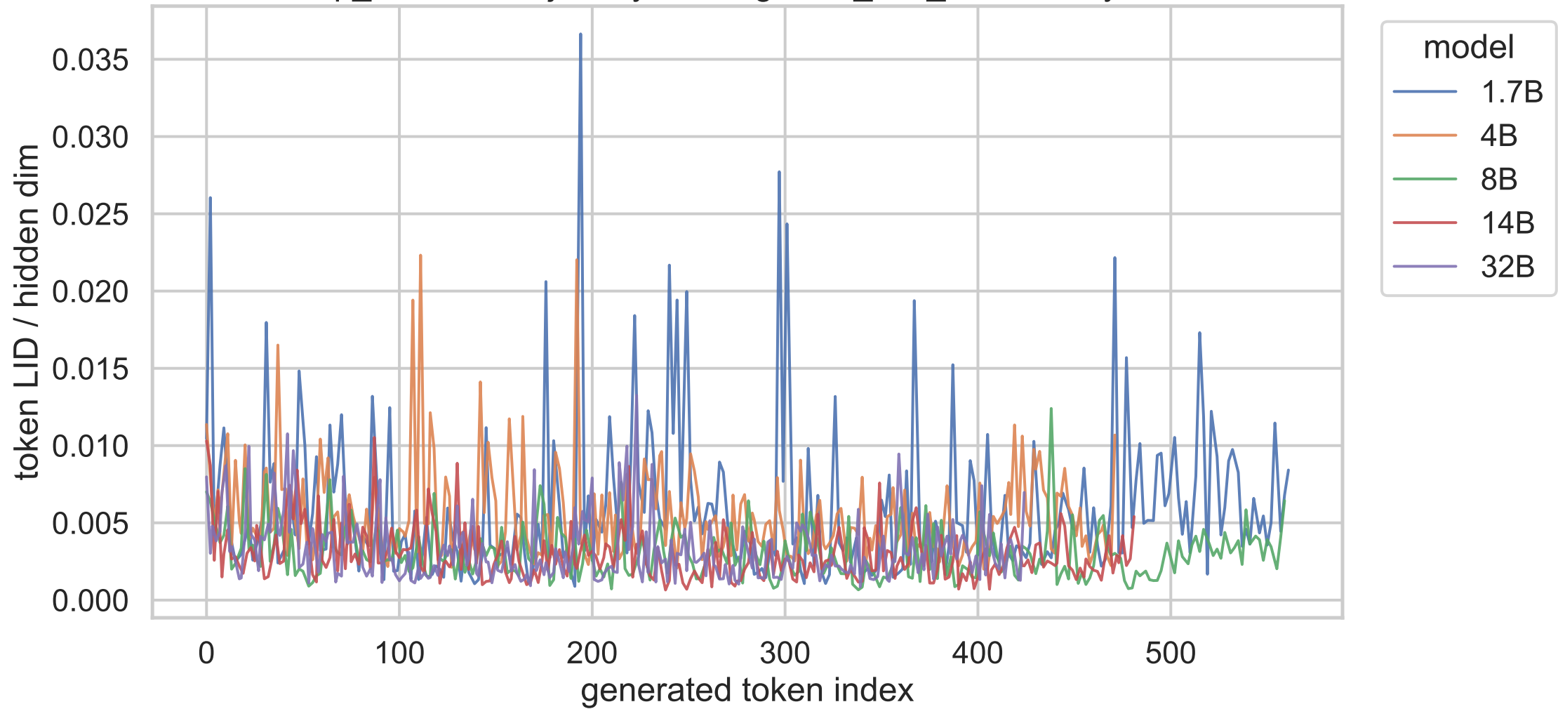
exp_c shared trajectory, think, gsm8k_test_000007, layer 20
