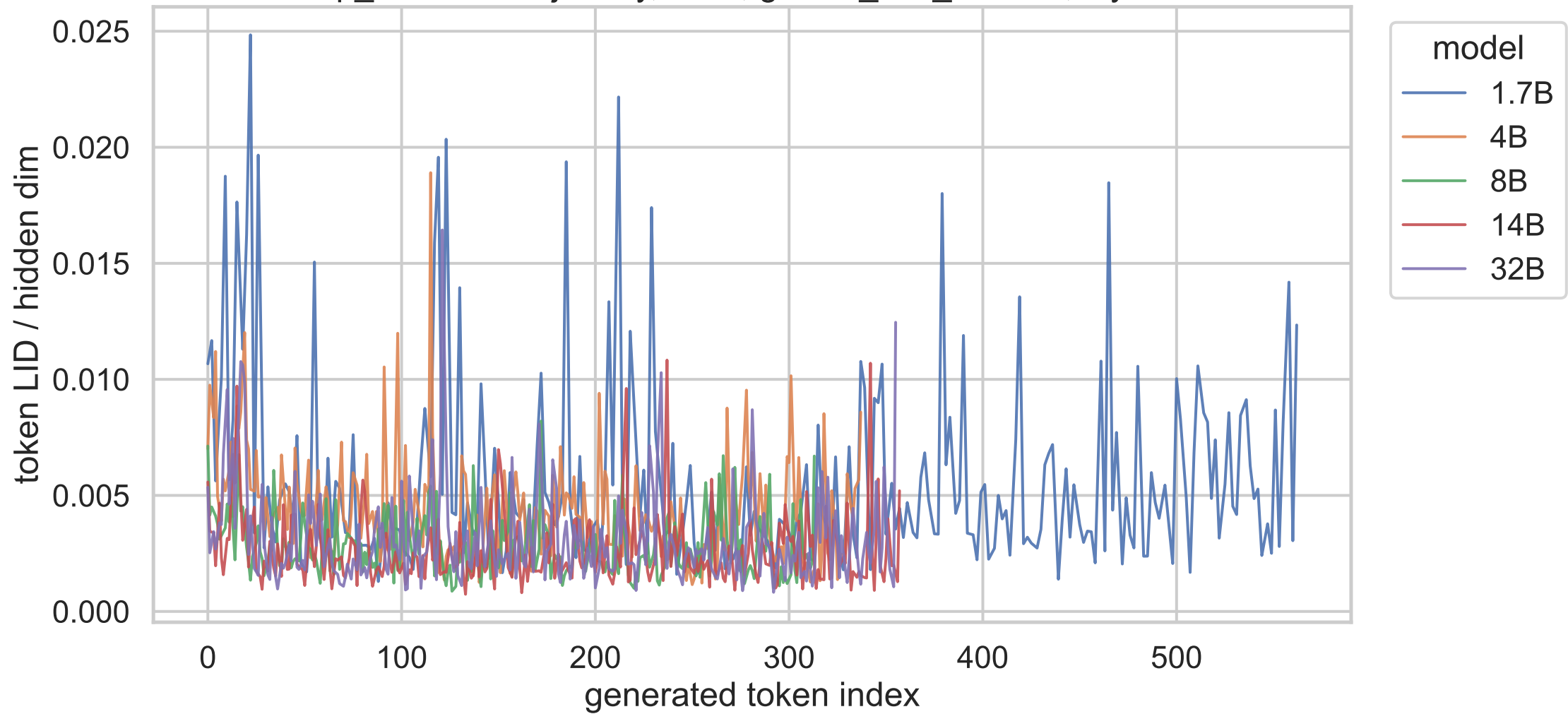
exp_c shared trajectory, think, gsm8k_test_000031, layer 20
