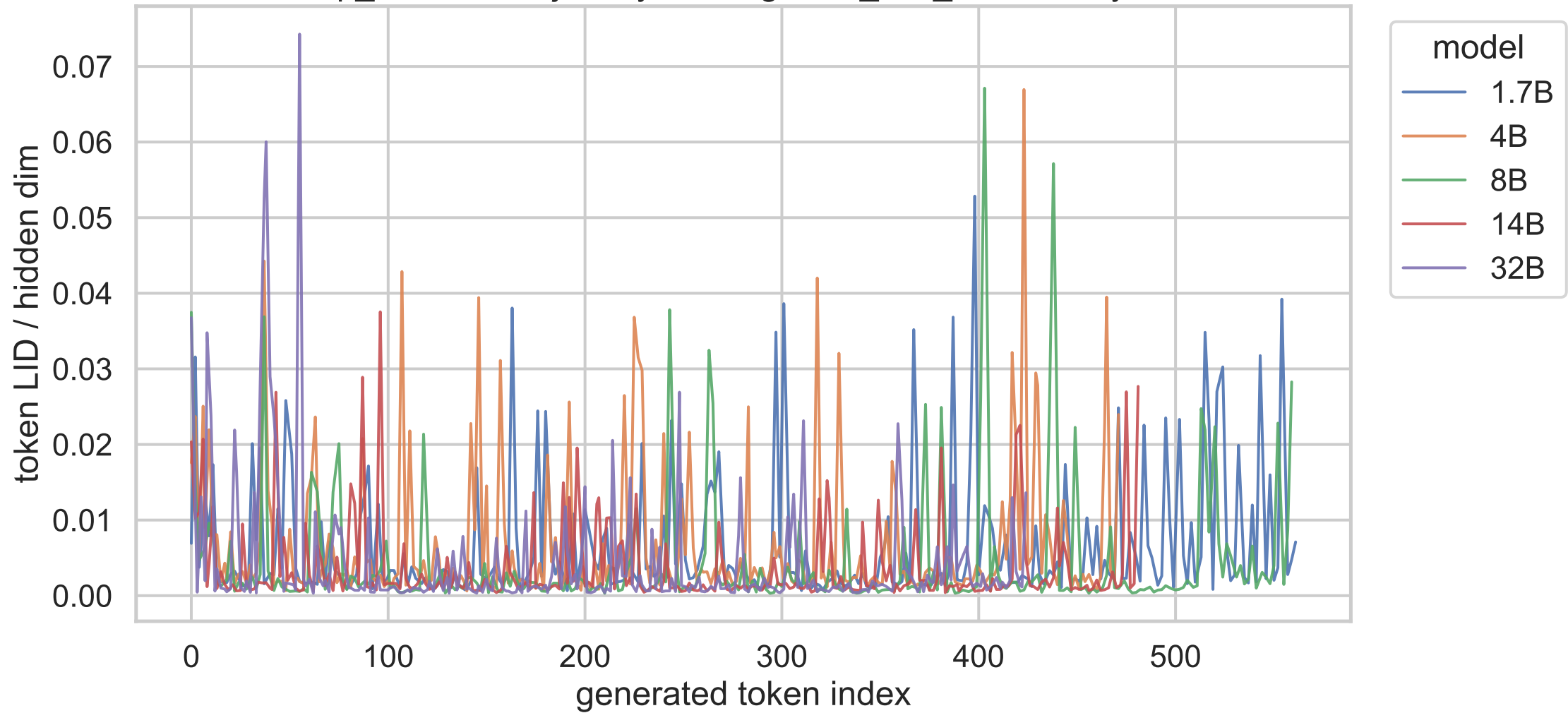
exp_c shared trajectory, think, gsm8k_test_000007, layer 6
